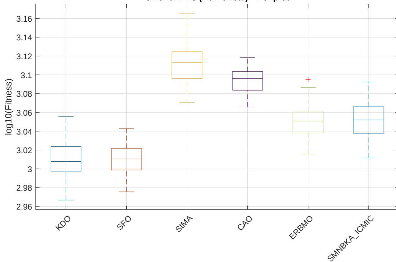
CEC2017 F8 (Numerical) - Boxplot
