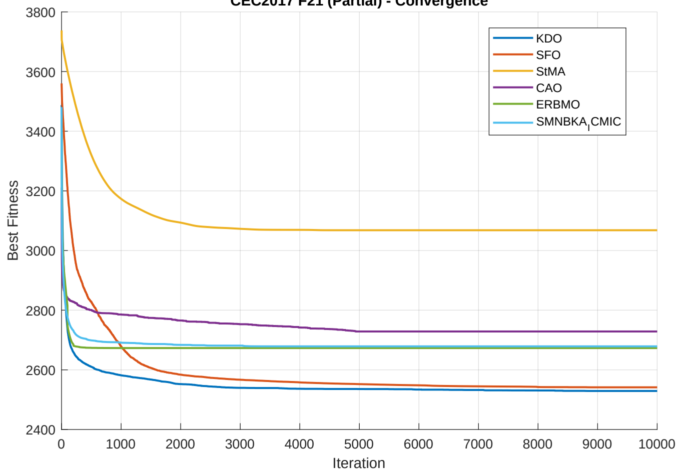
CEC2017 F21 (Partial) - Convergence
