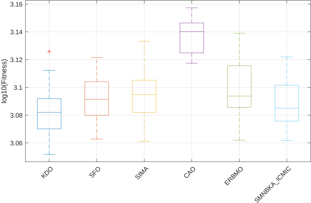
CEC2017 F11 (Numerical) - Boxplot
