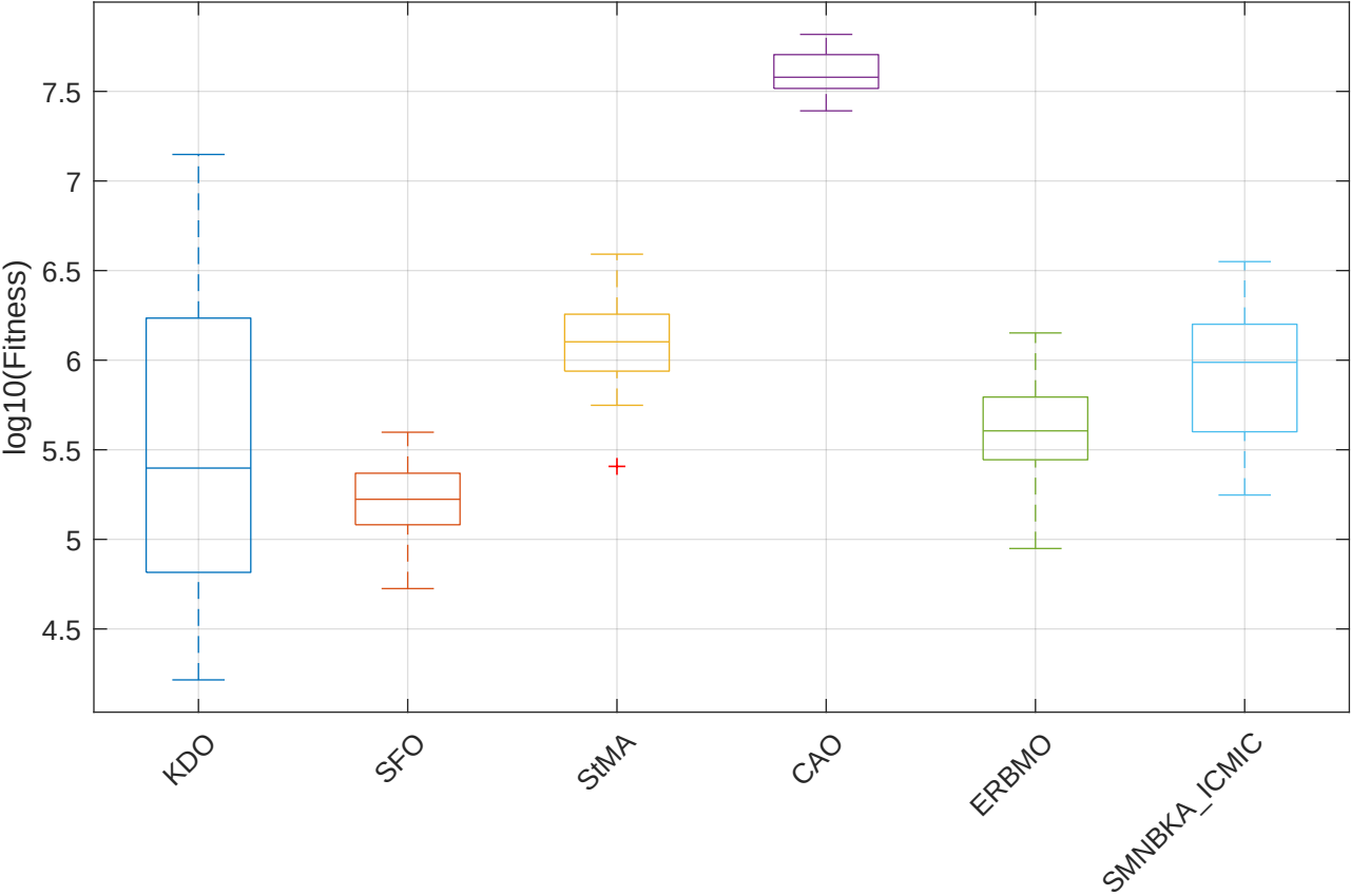
CEC2017 F12 (Numerical) - Boxplot
