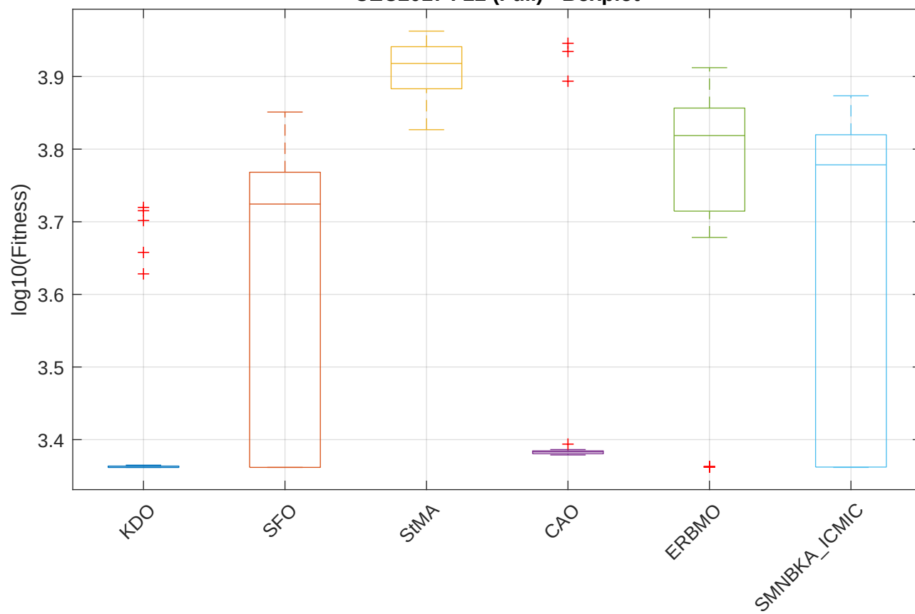
CEC2017 F22 (Full) - Boxplot
