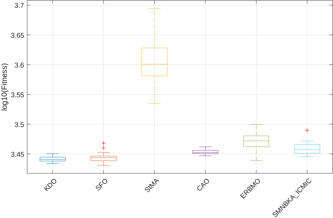
CEC2017 F23 (Numerical) - Boxplot
