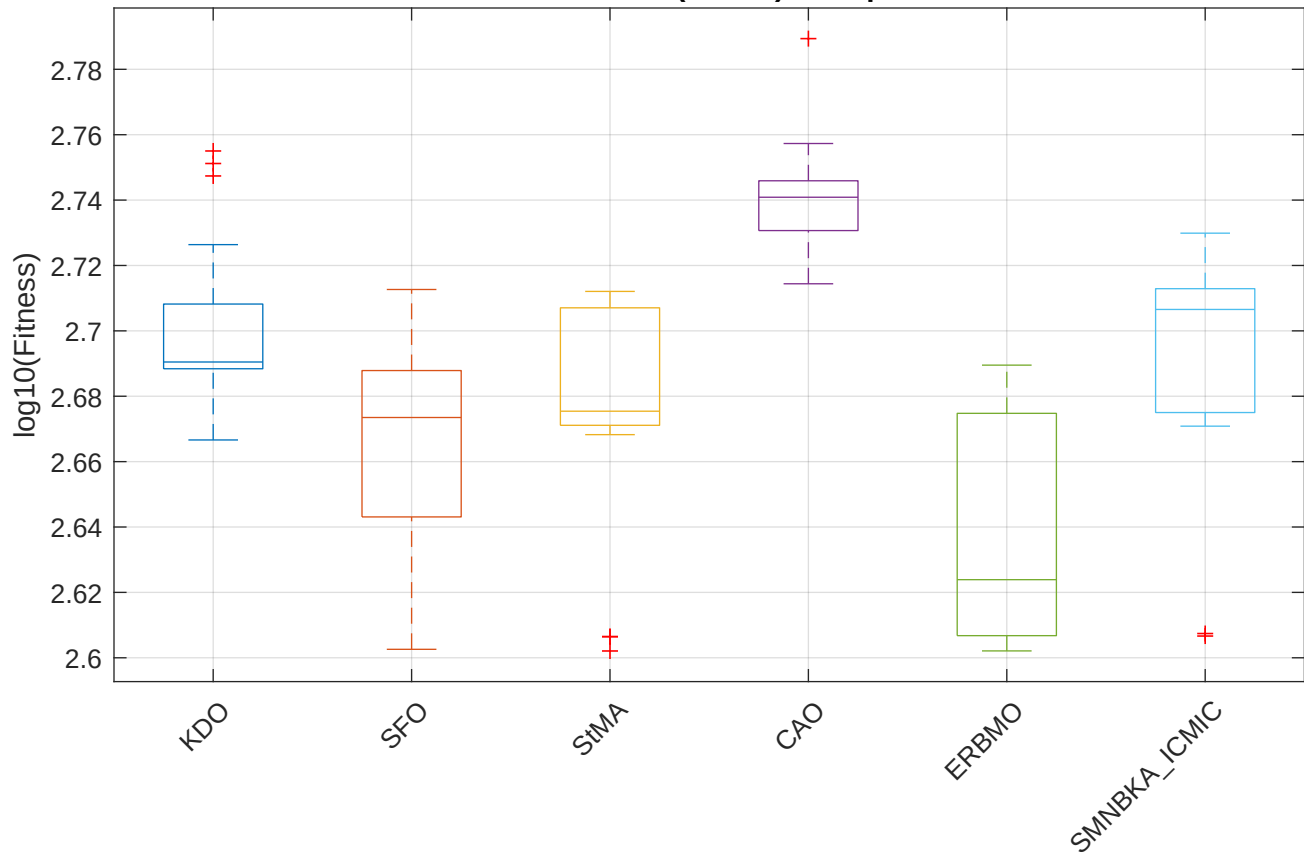
CEC2017 F4 (Partial) - Boxplot
