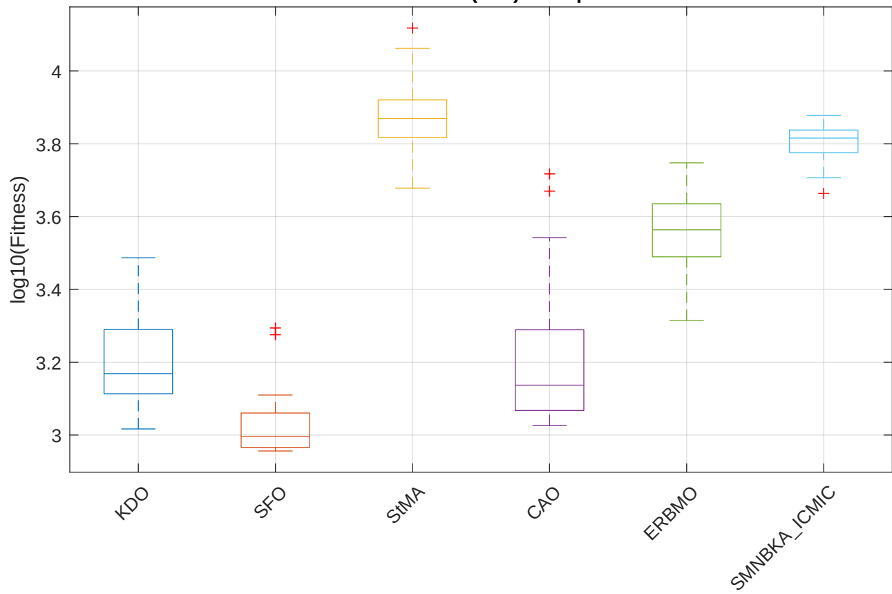
CEC2017 F9 (Full) - Boxplot
