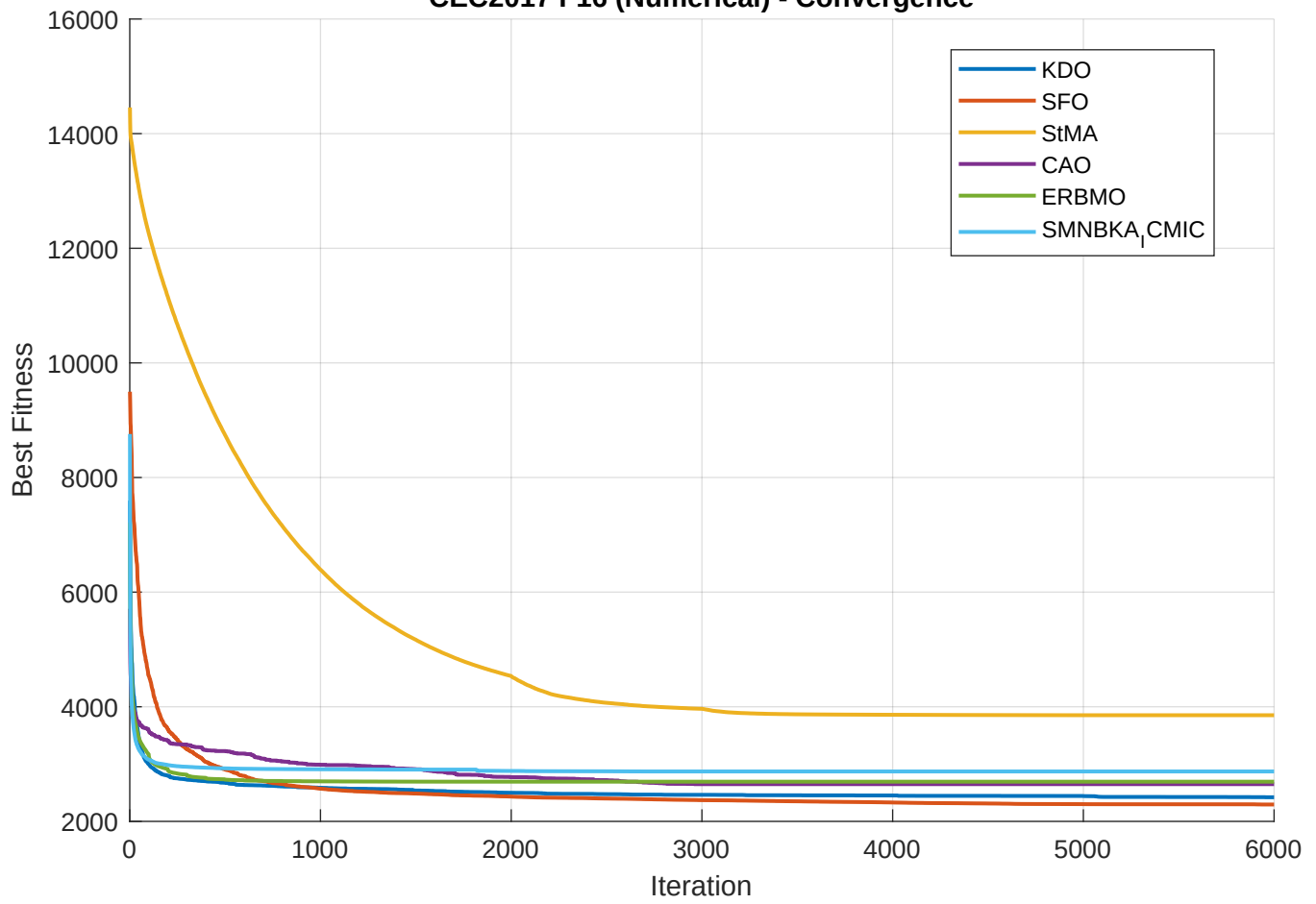
CEC2017 F16 (Numerical) - Convergence
