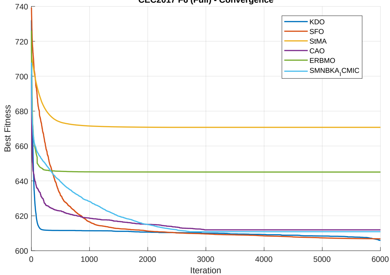
CEC2017 F6 (Full) - Convergence
