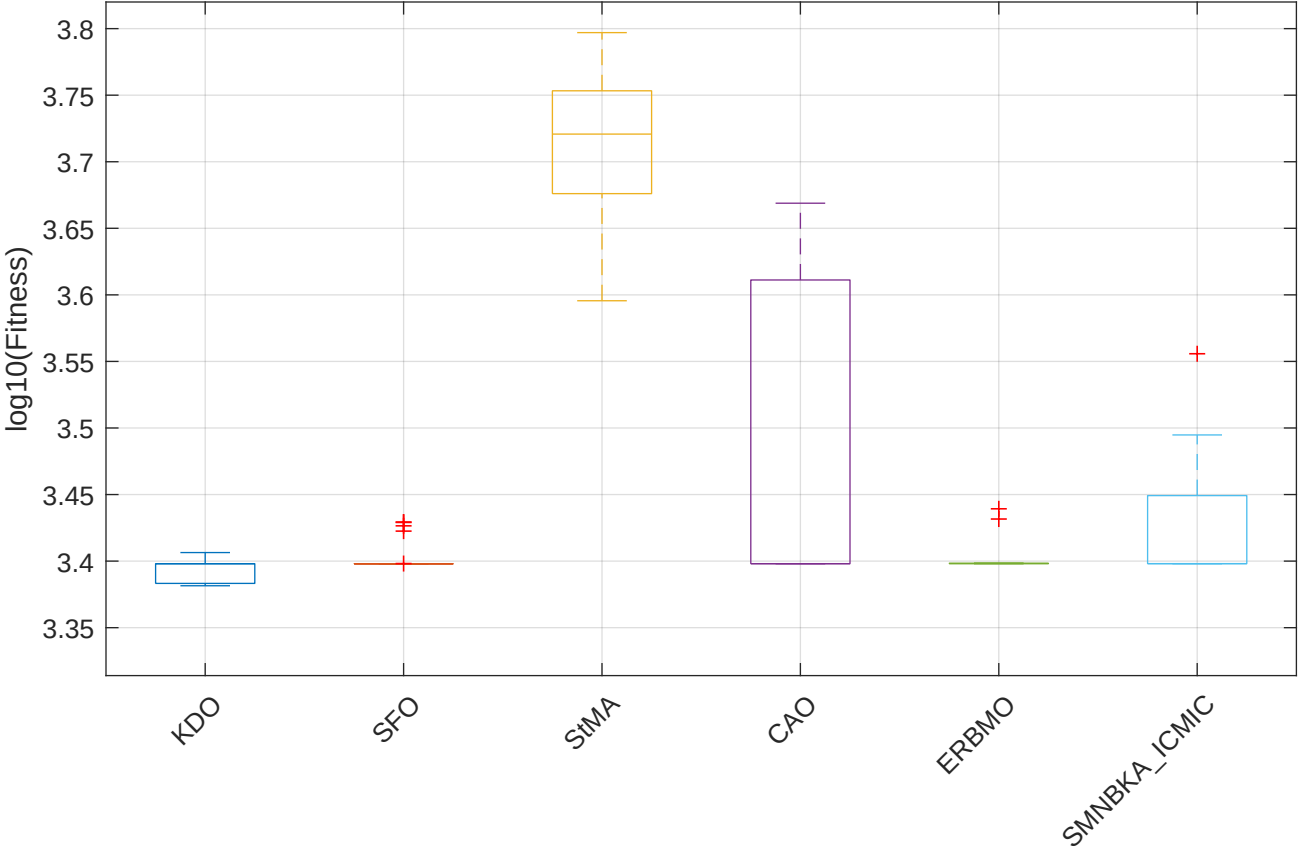
CEC2022 F10 (Numerical) - Boxplot
