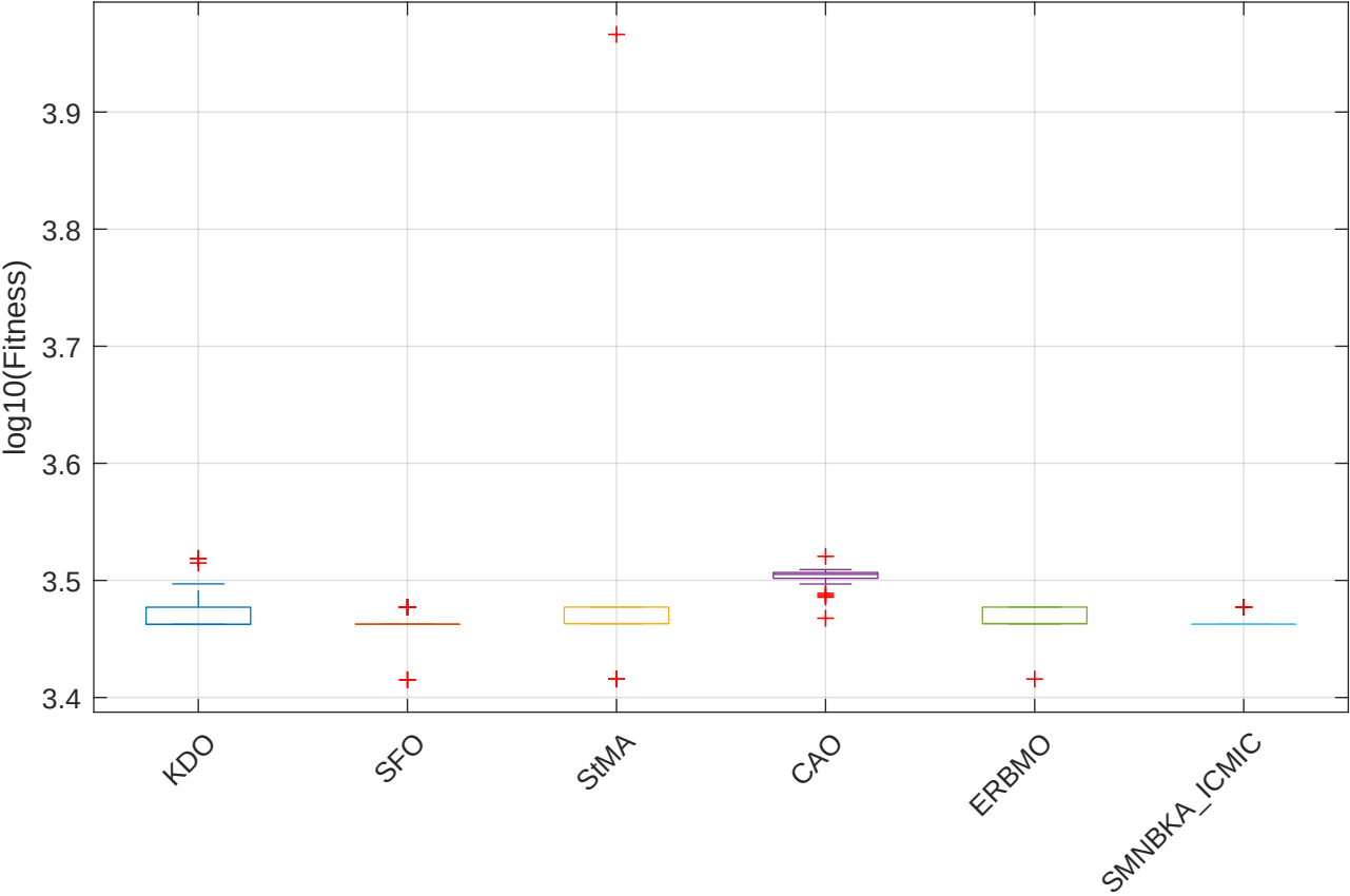
CEC2022 F11 (Numerical) - Boxplot
