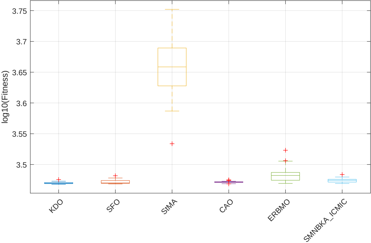
CEC2022 F12 (Numerical) - Boxplot
