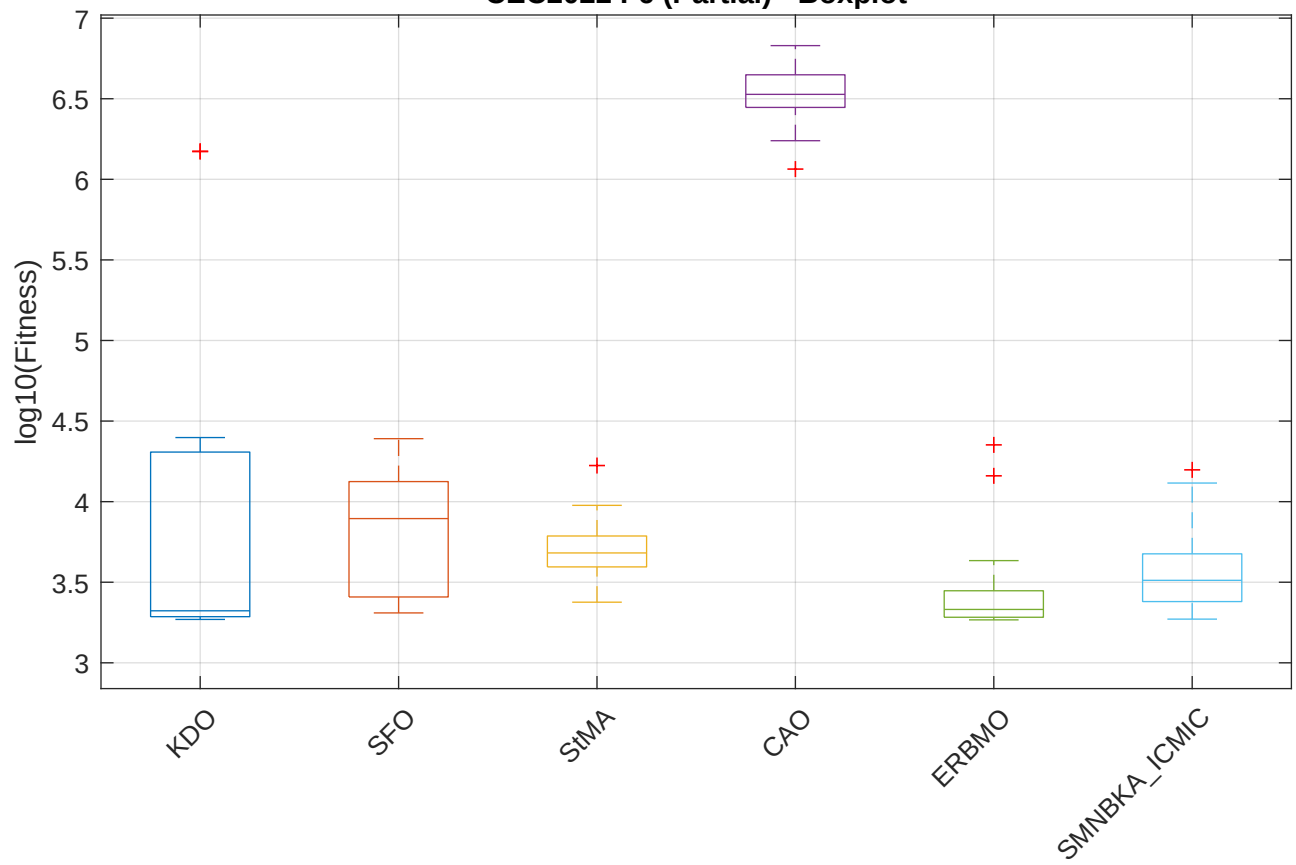
CEC2022 F6 (Partial) - Boxplot
