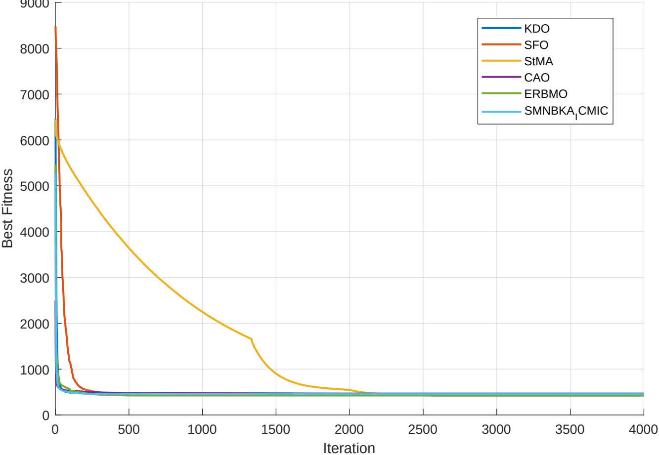
CEC2022 F2 (Full) - Convergence
