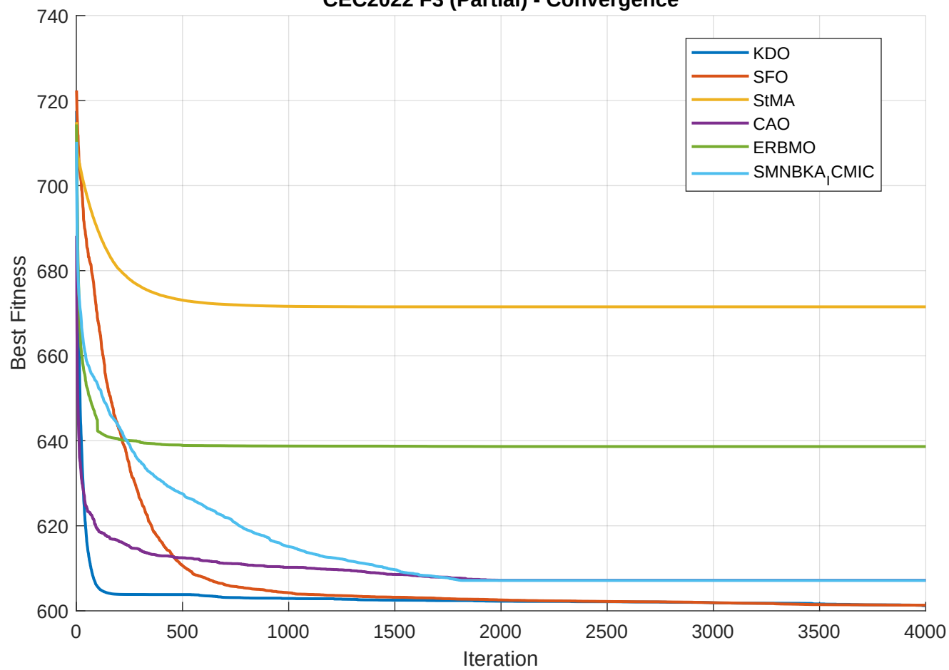
CEC2022 F3 (Partial) - Convergence
