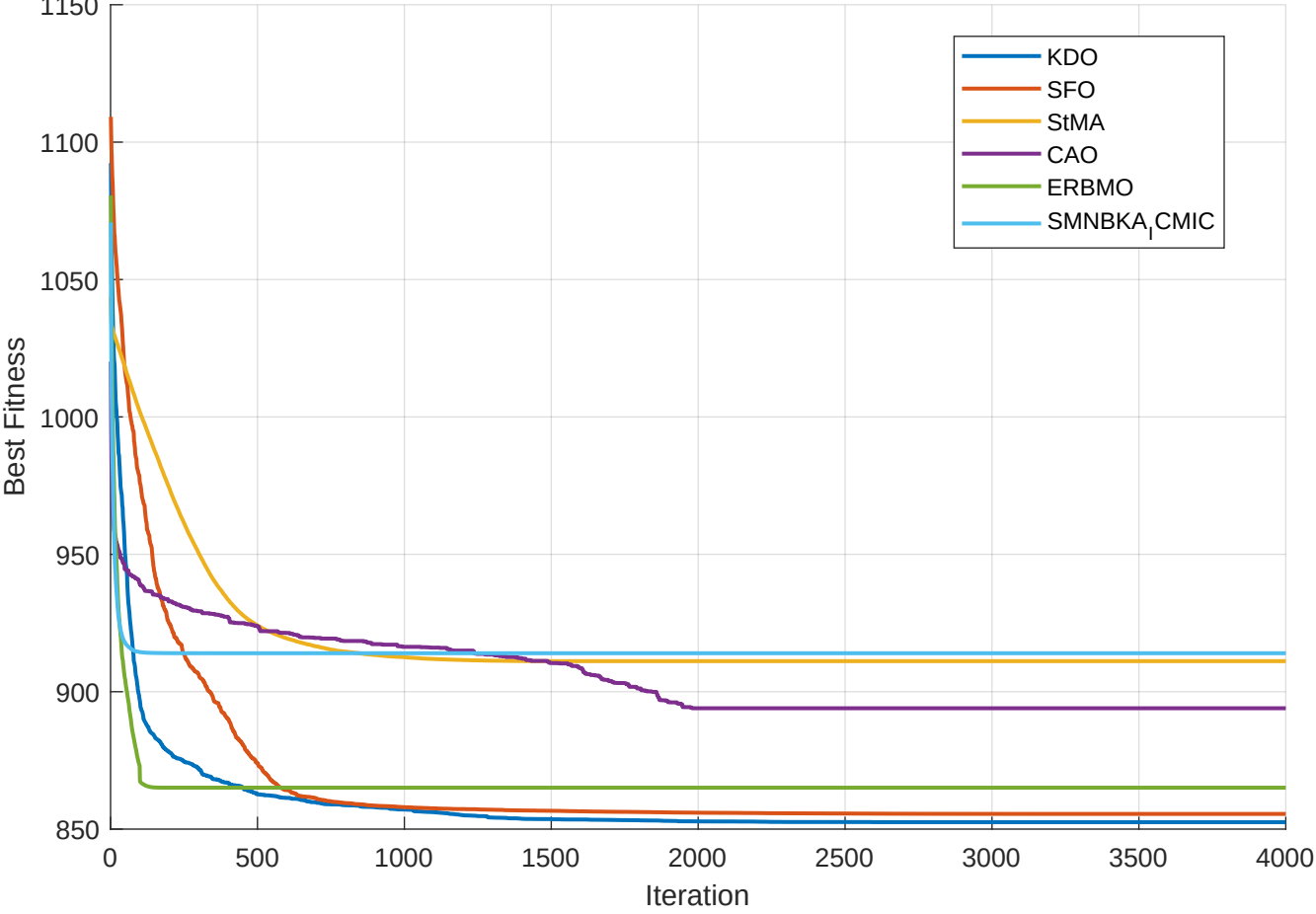
CEC2022 F4 (Full) - Convergence
