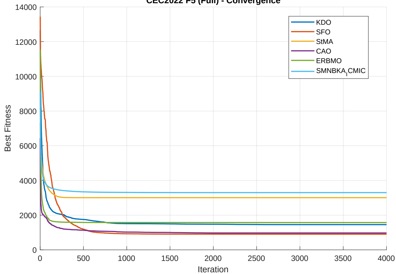
CEC2022 F5 (Full) - Convergence
