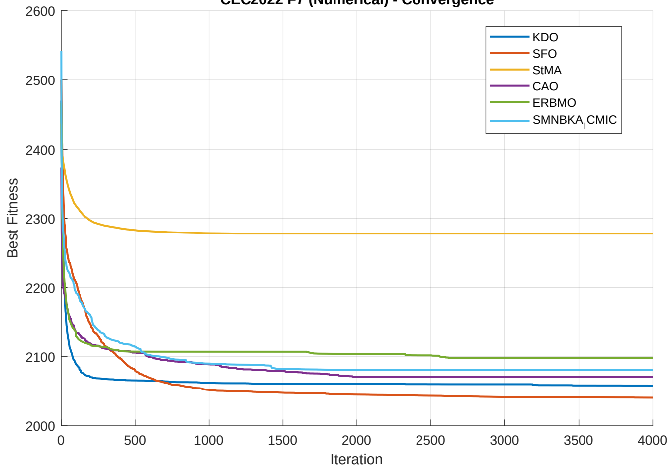
CEC2022 F7 (Numerical) - Convergence
