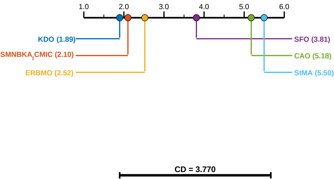
Critical Difference Diagram (Nemenyi, \alpha=0.05 )
