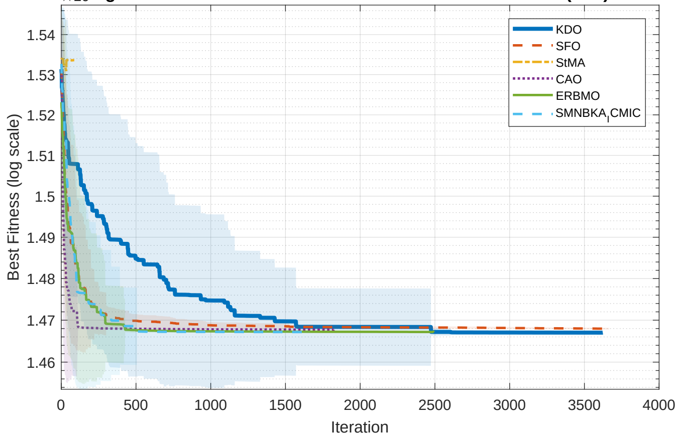
Convergence Curves - E3: Low Phase-Noise LC-VCO with PVT (11D) - HARD
