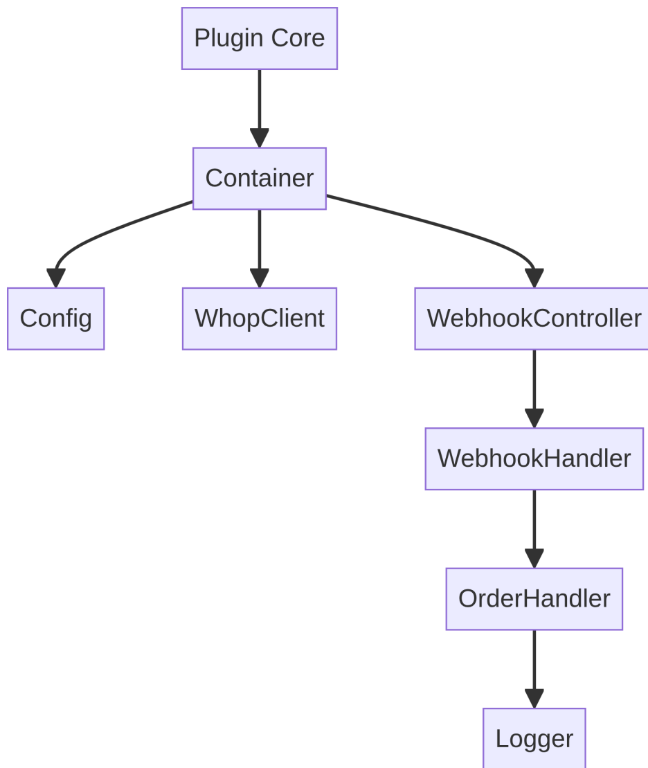
Diagram 2: Internal plugin architecture and service layers
