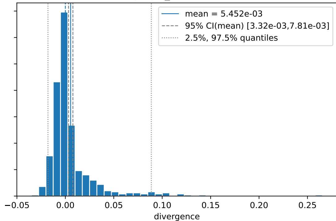
IPCW-plugin_km (n = 20000)
