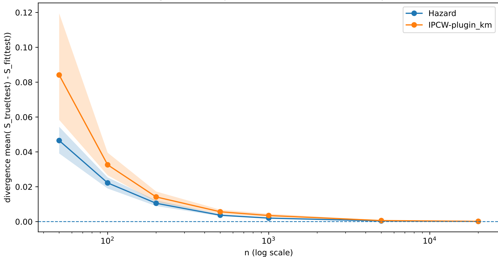
divergence vs sample size (mean and 95% bootstrap CI)
