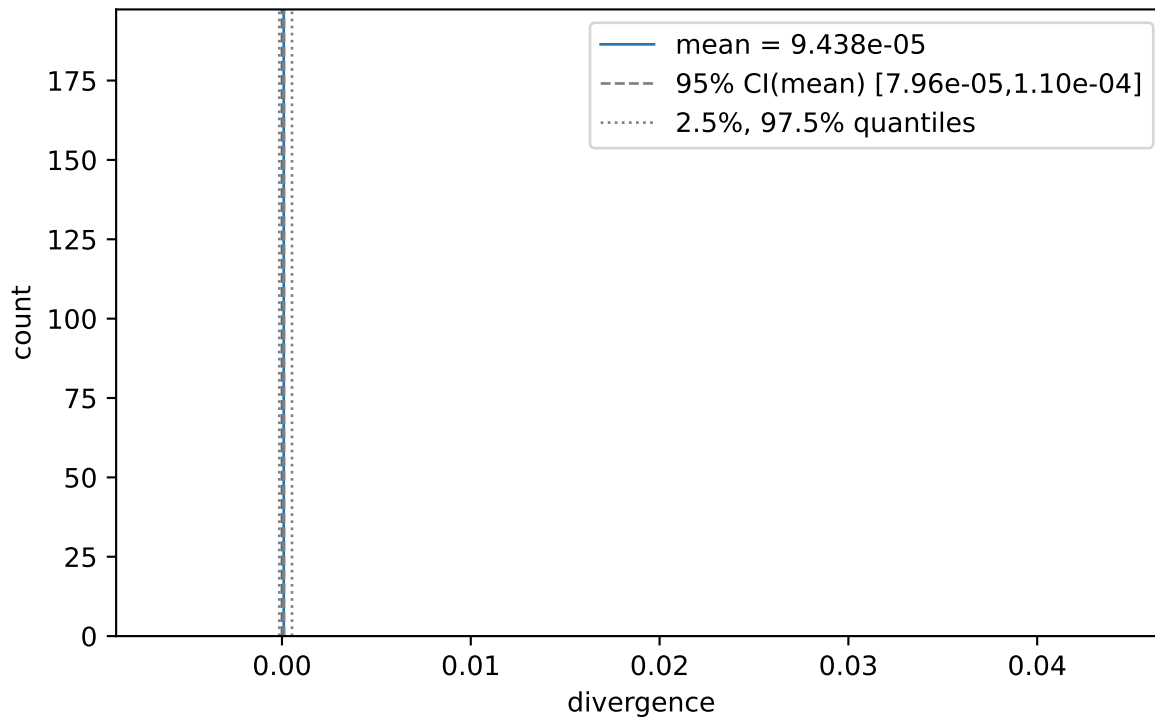
Hazard (n = 20000)
