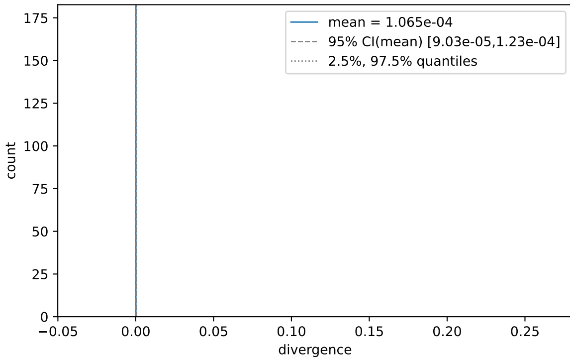
Hazard (n = 20000)
