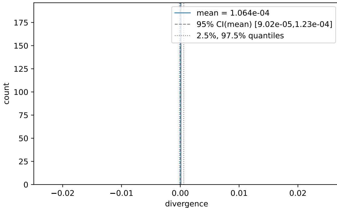
Hazard (n = 20000)
