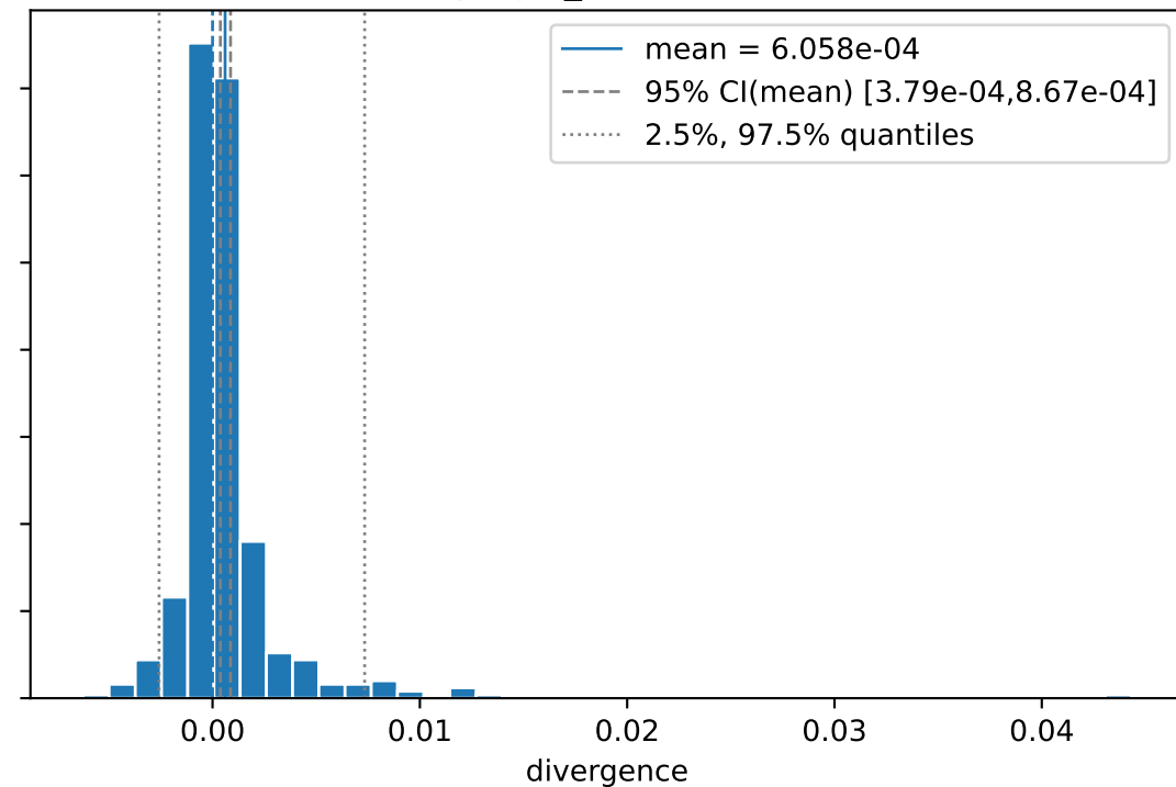
IPCW-plugin_km (n = 20000)
