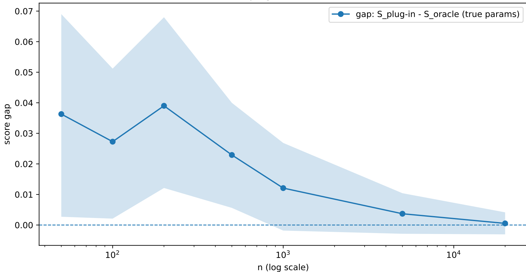
Nuisance estimation effect: plug-in vs oracle IPCW score (true model)
