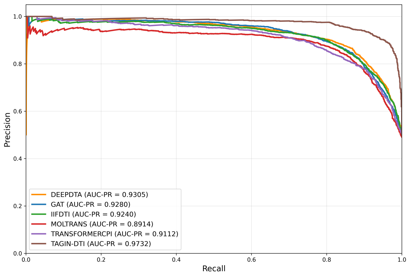
Precision-Recall Curves Comparison: Different Models on DrugBank Dataset
