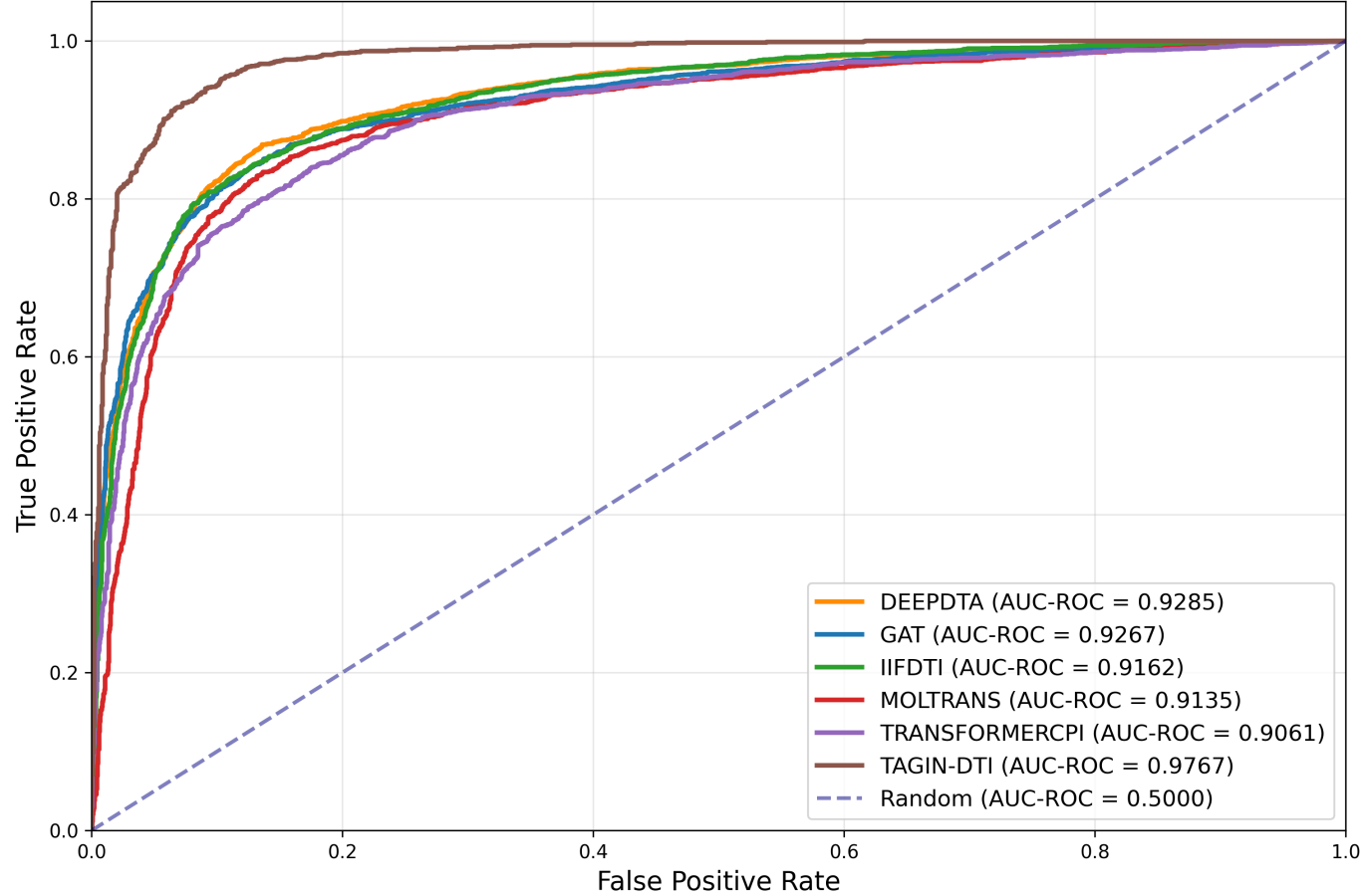
ROC Curves Comparison: Different Models on DrugBank Dataset
