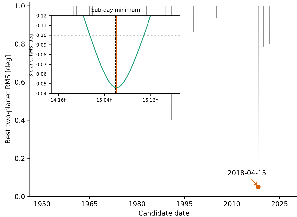
Blind planetary search, 1950-2026
