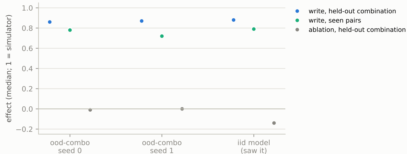
Unseen mass \times force combinations are computed, not looked up
