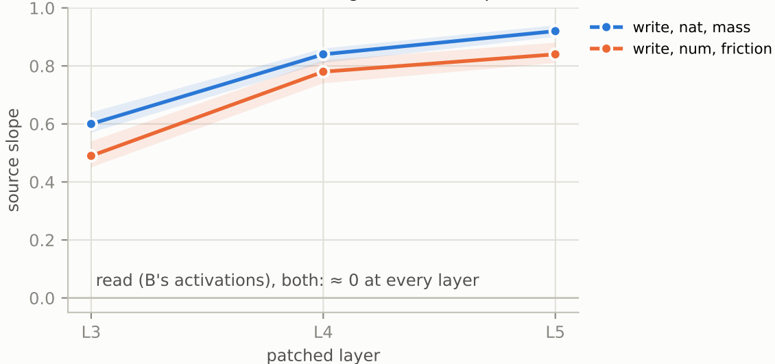
The write channel strengthens with depth
