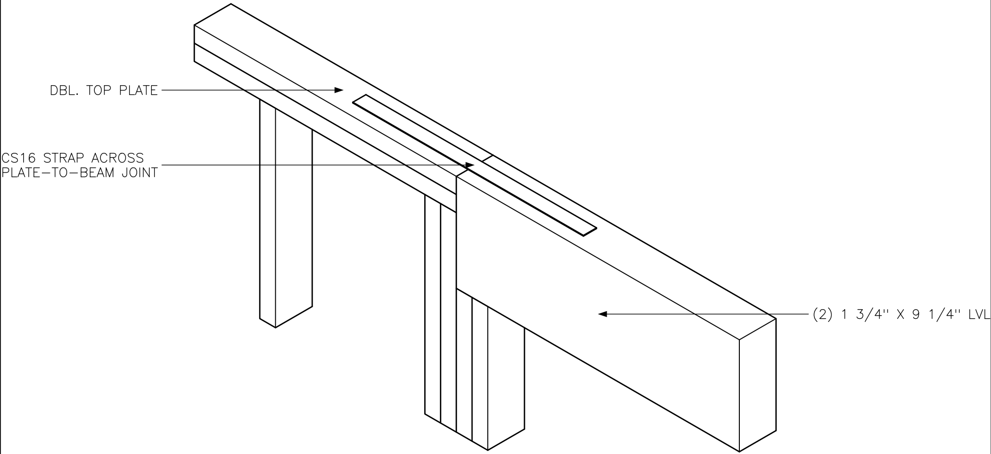
FLUSH BEAM AT TOP PLATE – ISO SCALE: NTS
