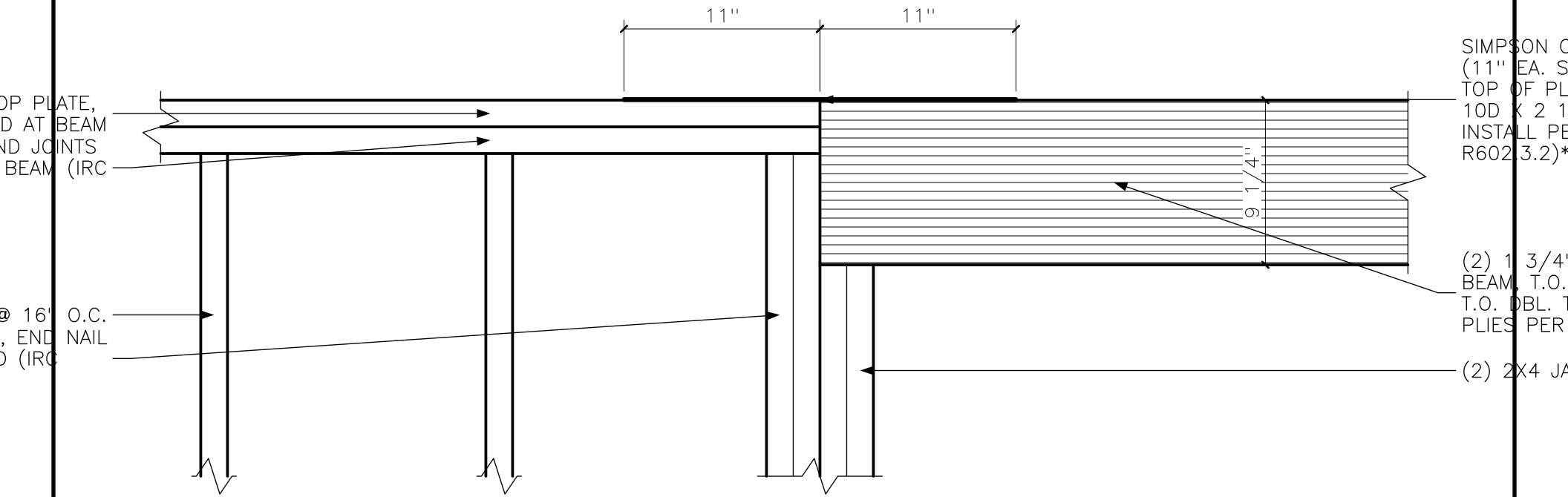
FLUSH BEAM AT TOP PLATE – ELEVATION SCALE: 1 1/2" = 1'-0"
