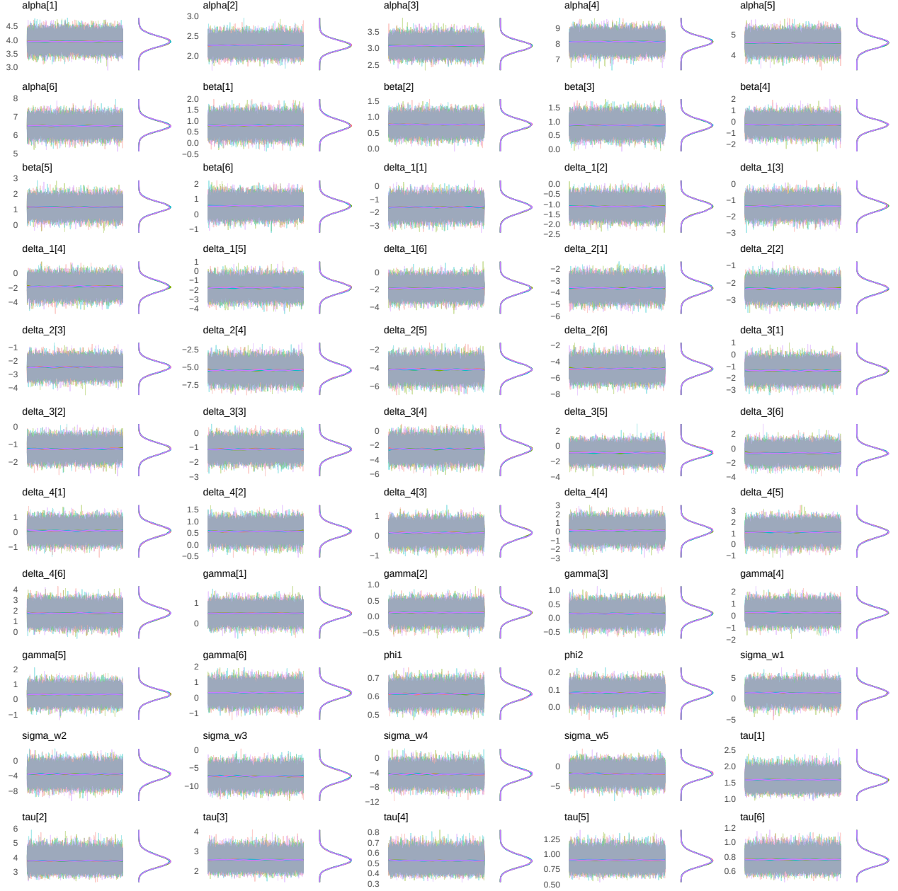
Figure 20: Trace with LOWESS fit (left) and posterior density (right) for every monitored parameter of the selected model. The horizontal axis is the iteration over the 20,000 retained draws, shared across all panels. Four chains overlaid after burn-in, only retained draws shown. The bracketed index on a parameter denotes the HSE region: 1 is Dublin and Midlands, 2 is Dublin and North East, 3 is Dublin and South East, 4 is Mid West, 5 is South West, 6 is West and North West. The four New Year window effects are numbered in temporal order: delta_1 the week two weeks before the New Year week, delta_2 the week before, delta_3 the New Year week (containing Jan 1), and delta_4 the week after.
