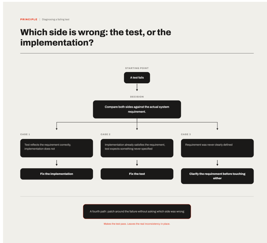
Figure 4.5: Decision flow for diagnosing a failing test: which side — the test or the implementation — holds the incorrect assumption.
