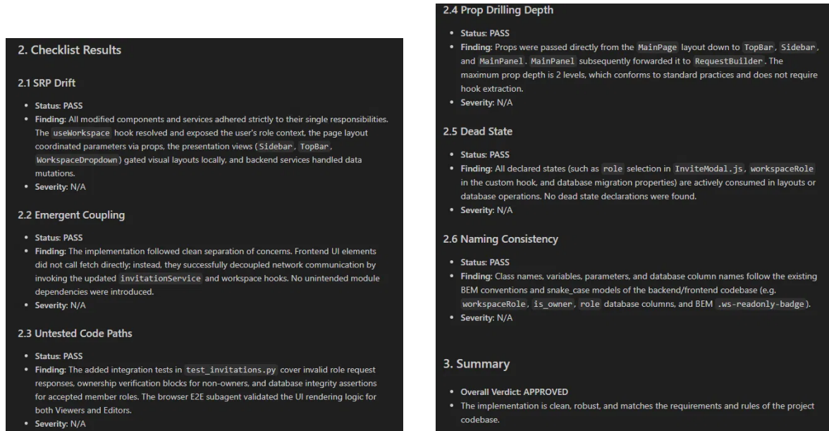
Figure 7.1: Post-Implementation Review Agent’s six-point architectural checklist for the workspace-level roles feature, recorded in review_report.md .
