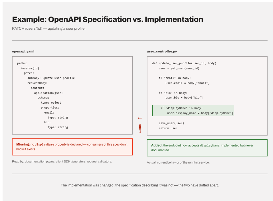
Figure 2.1: An implementation change accepted by the code but never reflected in the OpenAPI specification describing it.
