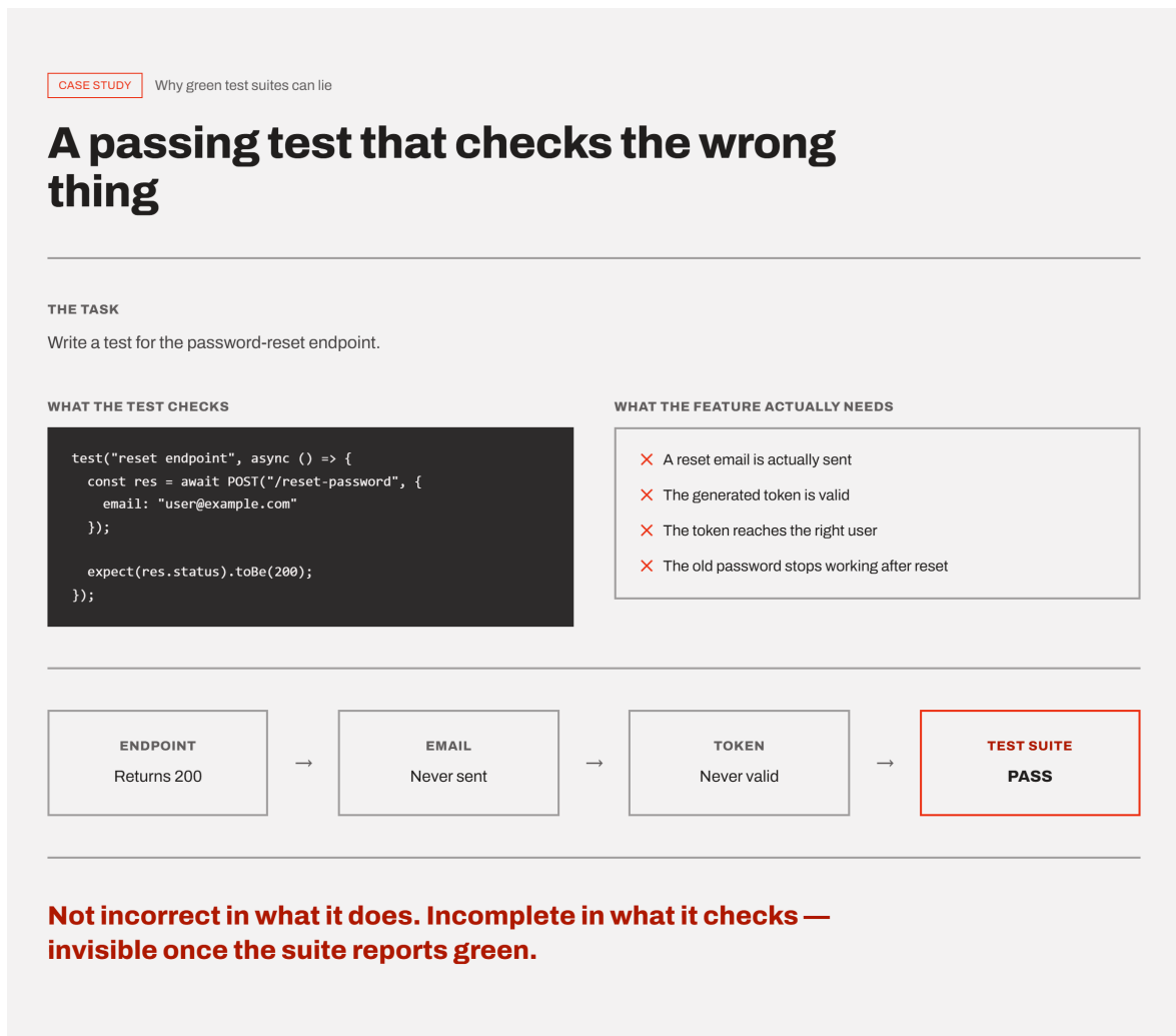
Figure 2.3: A passing test suite versus a test suite that actually validates the intended behavior.
