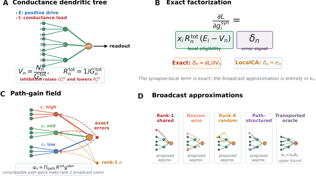
Figure 1: Model and credit assignment. (A) Conductance-based dendritic neuron. Nonnegative excitatory and inhibitory inputs drive distal compartments, which feed proximal branches and then the soma. In the shunting model, inhibitory conductance enters the total conductance in the denominator, so it changes the input resistance and the gain of upstream paths. (B) Exact credit versus LocalCA. Backpropagation supplies compartment-specific errors \partial L / \partial V_n at every dendritic level. LocalCA keeps the synapse-local eligibility term but replaces the exact compartment error with a low-bandwidth broadcast e_n that is routed down the tree. (C) Path gain through the tree. Exact backprop supplies a path-specific compartment error; rank-1 LocalCA replaces that field with one shared broadcast. (D) Broadcast approximations. Rank-1 shared broadcast, neuron-wise broadcast, rank- K random broadcast, path-structured broadcast, and transported oracle form a ladder from low-bandwidth local learning to an exact non-local upper bound.
