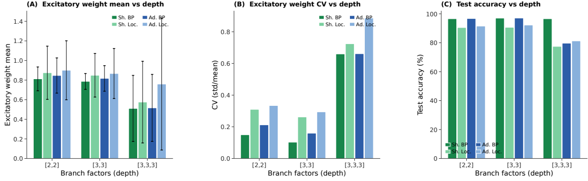
Figure S18: Synaptic weight statistics vs. dendritic depth (MNIST, 5 seeds/cell). (A) Excitatory weight mean (error bars = std). At [2,2] and [3,3], all four conditions cluster around 0.8–0.9; at [3,3,3] the means drop to \approx 0.5 –0.75 and the cross-seed spread grows, especially for additive LocalCA. (B) Coefficient of variation ( CV = \text{std}/\text{mean} ). At shallow/medium depth, LocalCA produces \sim 2\times higher CV than matched BP, but both remain well-behaved ( \leq 0.33 ). At the deepest network all four conditions jump to CV \approx 0.66 –0.88, with additive LocalCA the broadest. (C) MNIST test accuracy. BP tracks \sim 96 –97% at [2,2]/[3,3] and \sim 92 –95% at [3,3,3]. LocalCA stays within \sim 5 –6 pp of BP at shallow/medium depth but trails by \sim 15 –20 pp at [3,3,3], identifying depth as the remaining open challenge for this local rule. The qualitative ordering (shunting LocalCA tracks shunting BP more closely than additive LocalCA tracks additive BP) reinforces the manuscript claim that the conductance denominator is the key mechanistic ingredient.
