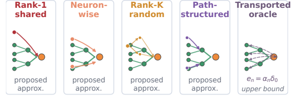
Figure 1: Model and credit assignment. (A) Conductance-based dendritic neuron. Nonnegative excitatory and inhibitory inputs drive distal compartments, which feed proximal branches and then the soma. In the shunting model, inhibitory conductance enters the total conductance in the denominator, so it changes the input resistance and the gain of upstream paths. (B) Exact credit versus LocalCA. Backpropagation supplies compartment-specific errors \partial L / \partial V_n at every dendritic level. LocalCA keeps the synapse-local eligibility term but replaces the exact compartment error with a low-bandwidth broadcast e_n that is routed down the tree. (C) Path gain through the tree. Exact backprop supplies a path-specific compartment error; rank-1 LocalCA replaces that field with one shared broadcast. (D) Broadcast approximations. Rank-1 shared broadcast, neuron-wise broadcast, rank- K random broadcast, path-structured broadcast, and transported oracle form a ladder from low-bandwidth local learning to an exact non-local upper bound.
