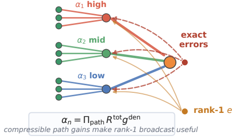
Figure 1: Model and credit assignment. (A) Conductance-based dendritic neuron. Nonnegative excitatory and inhibitory inputs drive distal compartments, which feed proximal branches and then the soma. In the shunting model, inhibitory conductance enters the total conductance in the denominator, so it changes the input resistance and the gain of upstream paths. (B) Exact credit versus LocalCA. Backpropagation supplies compartment-specific errors \partial L / \partial V_n at every dendritic level. LocalCA keeps the synapse-local eligibility term but replaces the exact compartment error with a low-bandwidth broadcast e_n that is routed down the tree. (C) Path gain through the tree. Exact backprop supplies a path-specific compartment error; rank-1 LocalCA replaces that field with one shared broadcast. (D) Broadcast approximations. Rank-1 shared broadcast, neuron-wise broadcast, rank- K random broadcast, path-structured broadcast, and transported oracle form a ladder from low-bandwidth local learning to an exact non-local upper bound.
