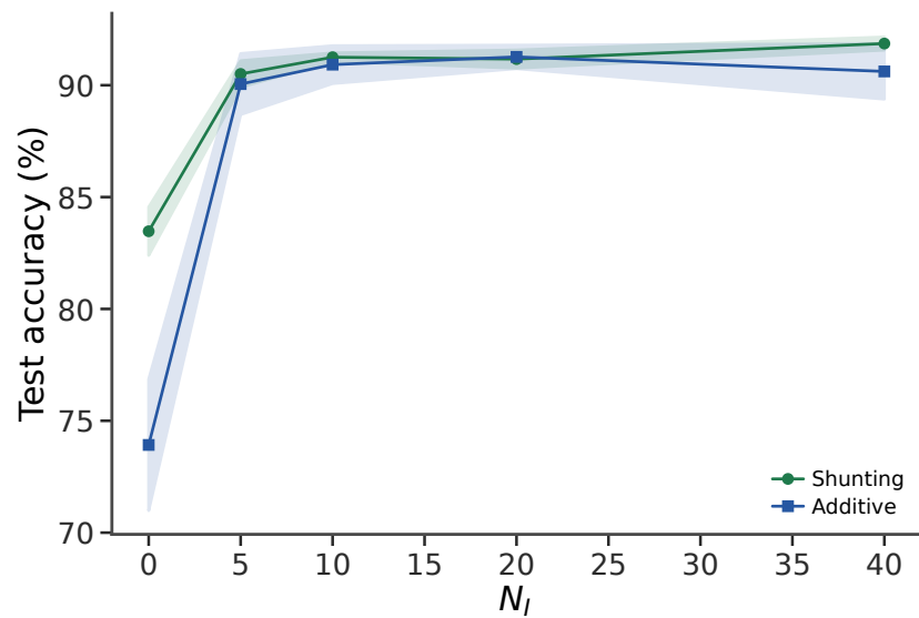
MNIST N_I sweep (detail)
