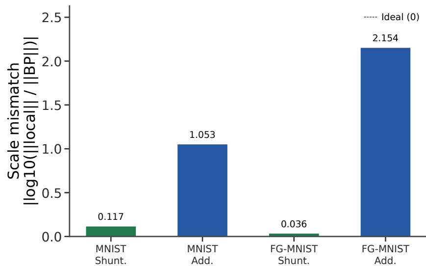
Scale mismatch
