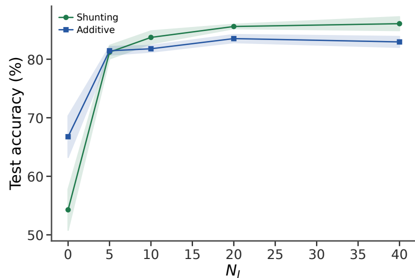
Noise resilience ( N_I detail)
