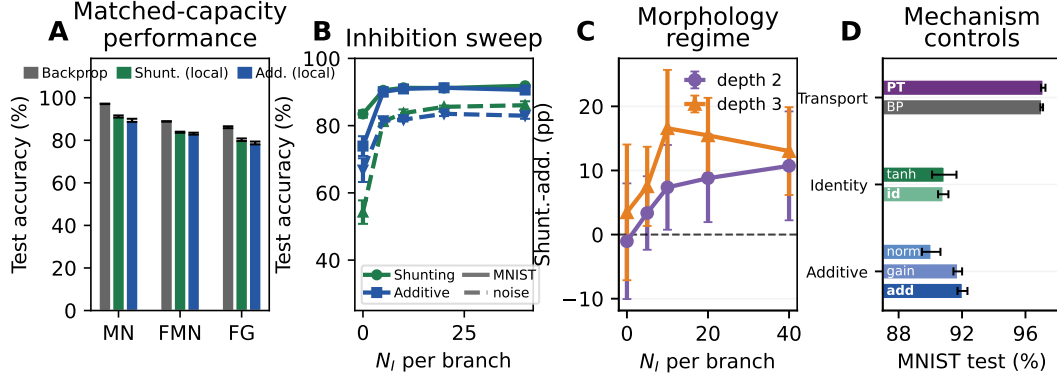
Figure 4: Matched-capacity performance and regime dependence. (A) Matched shunting backpropagation reference vs. matched-width/scalar-fallback 5F LocalCA; MN, FMN, and FG denote MNIST, Fashion-MNIST, and figure-ground MNIST. Additive backpropagation references are reported in Table S8 where matched five-seed runs are available. (B) Inhibitory dose-response. (C) Descriptive morphology-by-inhibition performance; the detailed map and its initialization limitation are in Appendix Fig. S11. (D) MNIST controls: backpropagation (BP), exact path transport (PT), identity vs. learned tanh activation, and additive gain/normalization variants. Values/protocols: Table S8; Appendix A. Error bars denote \pm 1 s.d.
