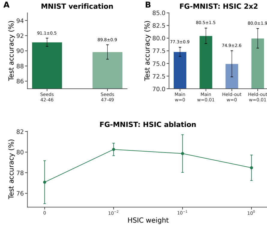
Figure S6: Verification and seed robustness (supplementary). (A) MNIST verification: repeat runs on main seeds (42–46) yield 91.1 \pm 0.5\% ; held-out seeds (47–49) yield 89.8 \pm 0.9\% , showing robustness across random seeds. (B) Matched figure-ground MNIST HSIC control: both main seeds (42–46) and held-out seeds (47–49) compare HSIC weight 0 against 0.01. (C) HSIC weight ablation on figure-ground MNIST: moderate weights (0.01–0.1) perform best.
