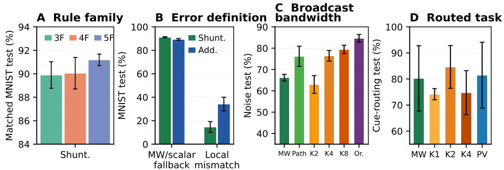
Figure S1: Detailed rule and feedback controls. (A) Within-shunting eligibility-rule ablation: 3F, 4F, and 5F. (B) Error-source ablation: submitted matched-width/scalar-fallback feedback vs. local mismatch. (C) Feedback-construction ladder on noise resilience: MW submitted feedback, recursive Path, random low-rank K2/K4/K8, and transported Oracle. (D) Cue routing: MW, random low-rank K1/K2/K4, and pathway-vector feedback.
