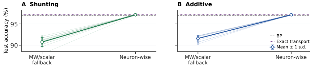
Figure 5: Preserving neuron identity closes the 3F MNIST gap. Replacing matched-width/scalar-fallback feedback by one soma coordinate shared over that neuron’s compartments improves every paired seed in both architectures ( n=15 ). Lines are seeds; large points and bars are mean \pm 1 s.d. BP and exact transport are matched references. The cross-architecture comparison is descriptive because the standard aliases use different gate-initialization policies; the paired substitution within each panel is causal. The explicit policy factorial is in Appendix Table S5; rule, rank, and routed-task controls are in Appendix Figs. S1 and S13 and Tables S4, S7, and S19.
