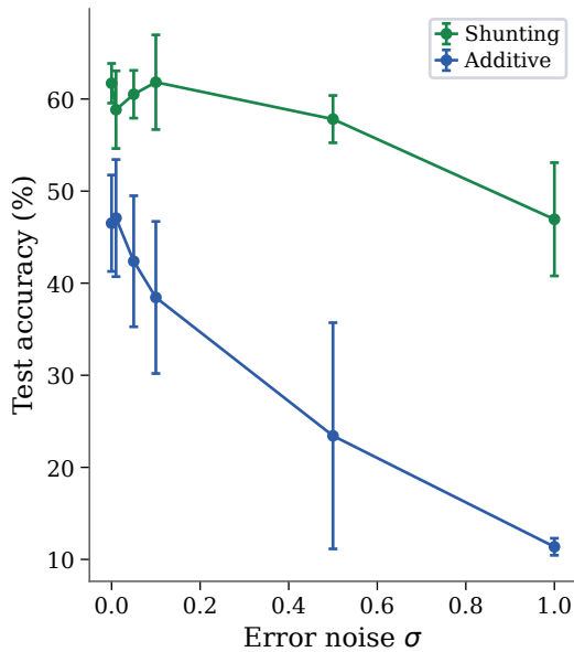
B Shunting tolerates noisy broadcasts
