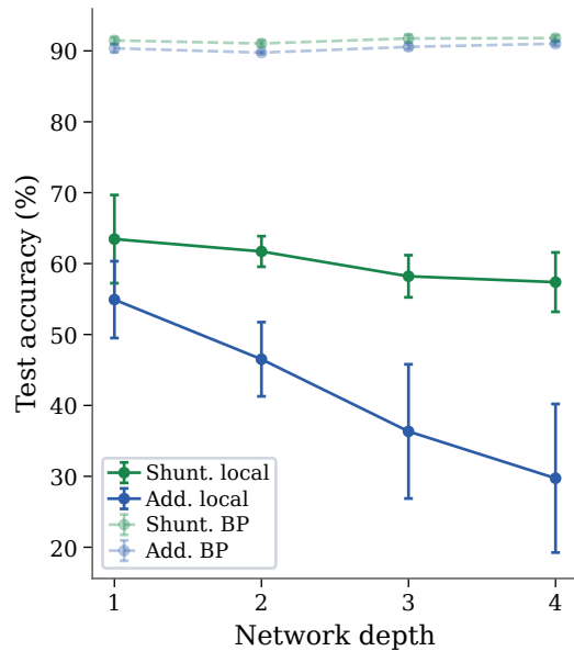
A Shunting degrades more gracefully with depth
