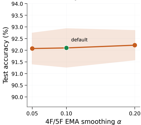
B 5F is moderately robust to EMA rate
