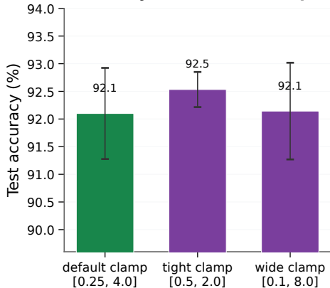
A 4F is not overly sensitive to clamp bounds
