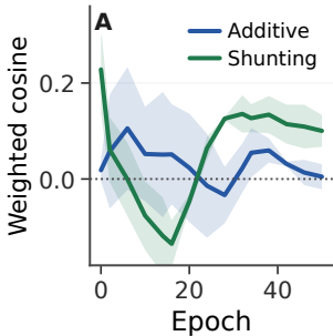
Alignment
