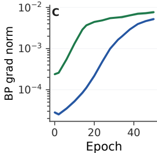
Backprop signal
