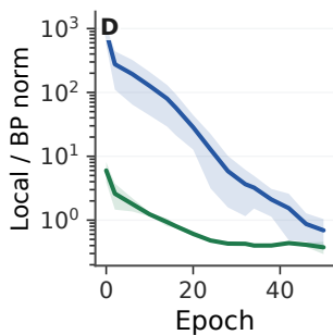
Scale mismatch
