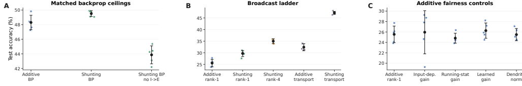
Figure S9: CIFAR-10 control ladder in the compact direct-I-stream family. (A) Matched backprop ceilings. With nonnegative inputs and a nonlinear decoder, shunting slightly exceeds additive under standard training, and removing learned I-to-E conductance lowers the shunting ceiling. (B) Broadcast ladder. Rank-1 broadcast remains weak on this harder dataset, rank-4 improves partially, and exact transported error nearly reaches the shunting backprop ceiling. (C) Additive fairness controls. Input-dependent gain, running-stat gain, learned gain, and dendritic normalization do not rescue additive rank-1 broadcast. This figure is a harder-data diagnostic, not a claim of competitive CIFAR-10 benchmarking.
