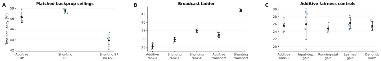
Figure S9: CIFAR-10 control ladder in the compact direct-I-stream family . (A) Matched backprop ceilings. With nonnegative inputs and a nonlinear decoder, shunting slightly exceeds additive under standard training, and removing learned I-to-E conductance lowers the shunting ceiling. (B) Broadcast ladder. Rank-1 broadcast remains weak on this harder dataset, rank-4 improves partially, and exact transported error nearly reaches the shunting backprop ceiling. (C) Additive fairness controls. Input-dependent gain, running-stat gain, learned gain, and dendritic normalization do not rescue additive rank-1 broadcast. This figure is a harder-data diagnostic, not a claim of competitive CIFAR-10 benchmarking.
