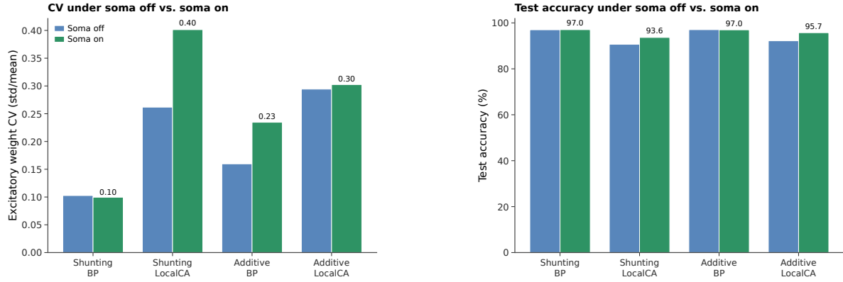
Figure S21: Excitatory-weight CV and MNIST accuracy under soma-off vs. soma-on (depth [3,3], 5 seeds/cell). (A) Coefficient of variation of excitatory weights for the four (core, strategy) cells; paired bars show soma-off (from Fig. S20) and soma-on (this sweep). Shunting + BP tightens slightly; shunting + LocalCA broadens; additive cells change little. (B) Matched MNIST test accuracy (sanity panel). BP accuracy is preserved or marginally improved; LocalCA accuracy is preserved for additive but drops \sim 3 pp for shunting, consistent with the CV widening in panel A.
