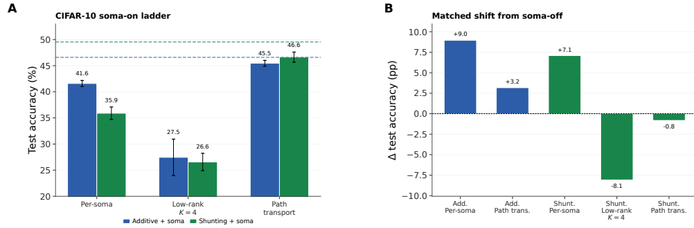
Figure S10: CIFAR-10 compact direct-I-stream depth-4 with somatic_synapses=true. (A) Absolute soma-on ladder on the compact direct-I-stream depth-4 family. Path transport stays strongest in both cores and remains near the matched backprop ceilings (dashed lines), while low-rank K=4 remains weak. (B) Matched shift from soma-off to soma-on for the conditions with a clean paired baseline. Soma helps additive strongly under per-soma and path transport, improves shunting per-soma, leaves shunting transported error close to its soma-off value, and worsens shunting low-rank K=4 . Additive low-rank K=4 is omitted from panel B because the soma-off mechanism package did not include that exact matched condition.
