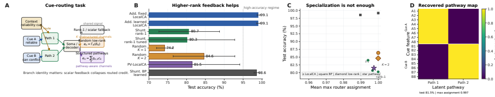
Figure S15: Structured feedback when rank-1 broadcast fails. (A) Cue-routing task schematic. Context determines which noisy cue is reliable on each trial, so different dendritic pathways should receive different teaching signals. (B) Five-seed comparison of rank-1, random low-rank, and pathway-structured feedback. Moving beyond rank-1 helps, while the best structured repair remains open. (C) Test accuracy vs. router specialization across learned-router conditions. High specialization alone does not guarantee success. (D) Recovered pathway assignments for a representative learned-router run. Cue-A and cue-B features segregate into separate latent pathways even when feedback quality, rather than router discreteness, is the limiting factor.
