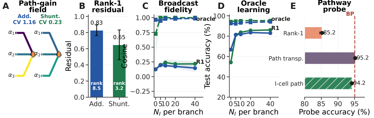
Figure 4: Mechanistic chain from path gains to learning. (A) Example dendritic path-gain field at matched inhibition, with measured MNIST CV annotated for additive and shunting networks. (B) Exact-error compressibility on MNIST: lower rank-1 residual and lower participation rank mean that a scalar broadcast is a better approximation. (C) Direct compartment-error fidelity on noise resilience. Solid lines compare rank-1 broadcast to the exact compartment error; dashed lines show the transported-error oracle. (D) Learning with the transported-error oracle. Improving the broadcast field recovers near-ceiling local learning, especially where rank-1 broadcast fails. (E) Compact inhibitory-path probe. In a one-layer noise-resilience test, exact path transport closes the rank-1 gap, and explicit inhibitory cells trained by the same local rule remain near the explicit-I backprop ceiling. Error bars denote \pm 1 s.d. across seeds.
