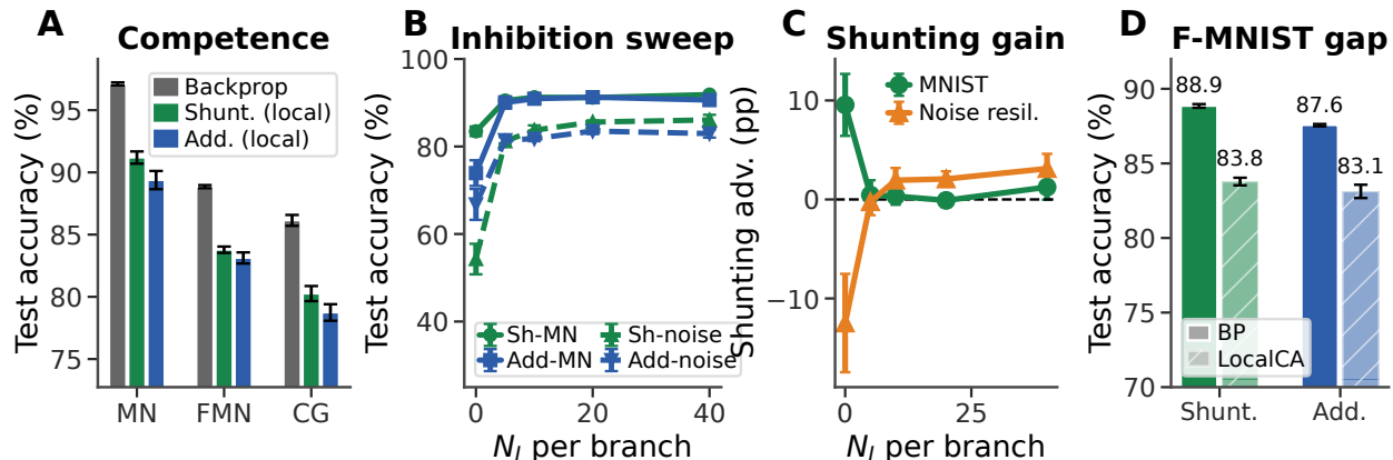
Figure 5: Capacity-calibrated competence and regime dependence. (A) Matched backprop ceilings vs. rank-1 5F LocalCA on MNIST, Fashion-MNIST, and context gating, including the matched additive context-gating rerun. (B,C) Inhibitory dose-response and shunting advantage on MNIST and noise resilience. (D) Fashion-MNIST confirms a smaller but consistent shunting advantage. Error bars denote \pm 1 s.d. across seeds.
