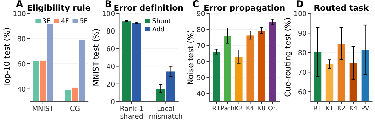
Figure 3: Local-rule and feedback-design axes. (A) The theorem-facing 3F update and the 4F attenuation proxy are weak practical optimizers in the completed local-competence sweeps; 5F is the strongest empirical wrapper. (B) The broadcast definition matters: on MNIST, rank-1 shared somatic error is strong, while a local-mismatch error surrogate fails. (C) On noise resilience, recursively propagating or increasing the rank of the error field closes much of the gap between rank-1 broadcast and exact path transport. (D) Cue routing probes a branch-specific regime: higher rank helps, while the current pathway-vector implementation is useful but not yet better than the best unstructured low-rank control. Error bars denote \pm 1 s.d. where five-seed summaries are available.
