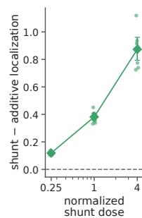
Cellwise contrast
