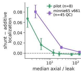
Cellwise contrast
