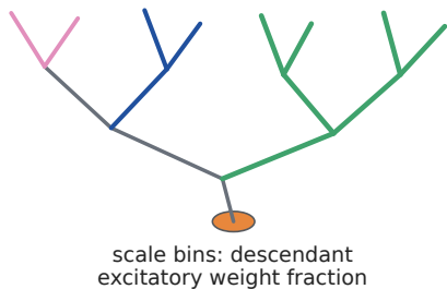
A Irregular-tree scale basis
