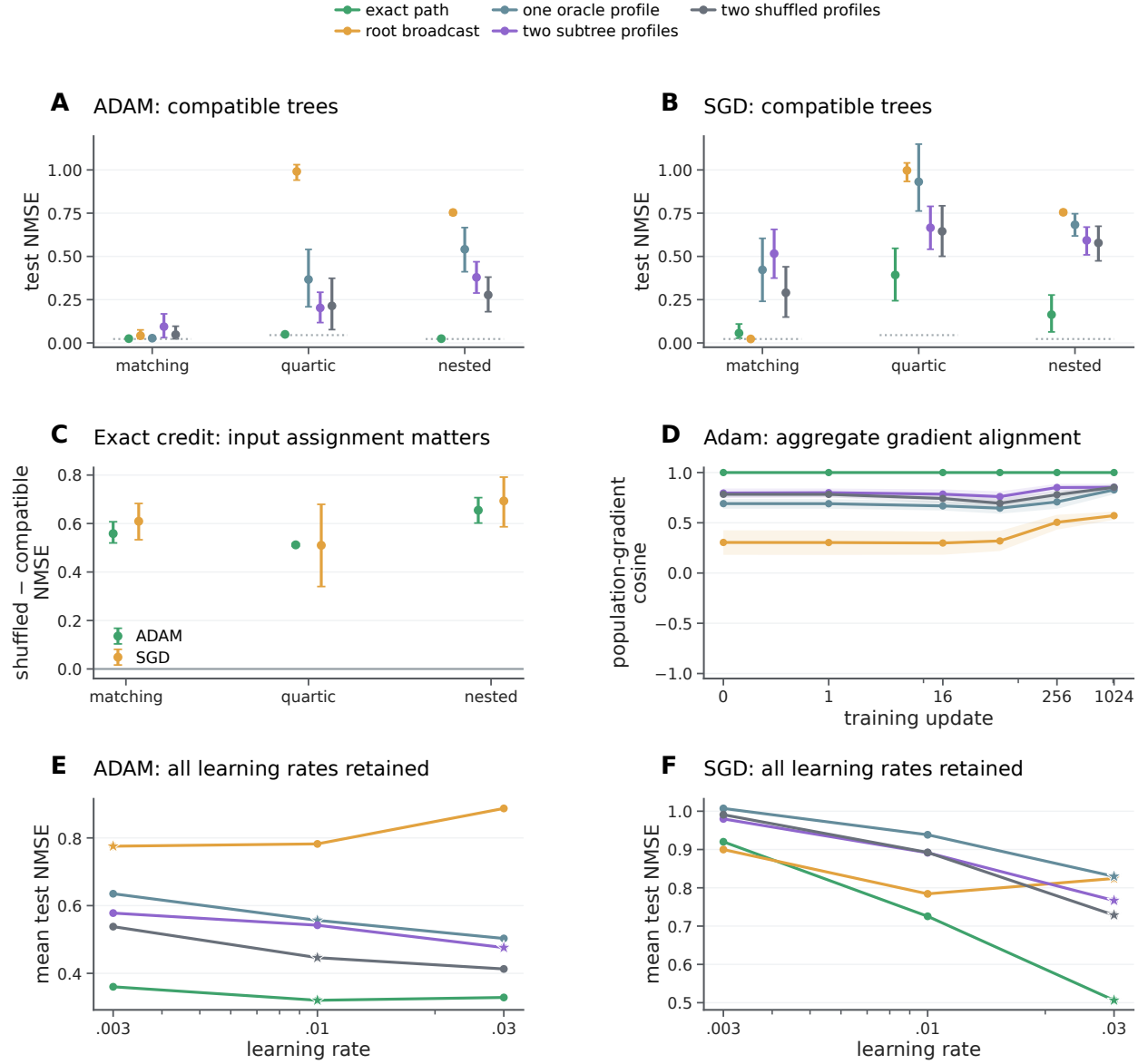
Figure S13: Task-dependent credit requirements in bounded multi-affine trees. A,B , Final test normalized mean squared error (NMSE) on oracle-compatible trees under Adam and stochastic gradient descent (SGD), respectively. Exact path, root broadcast, one oracle profile, two subtree profiles and two shuffled profiles share the forward model, initialization, examples and minibatches. Dotted segments mark known label-noise floors: 0.0225 for matching/nested tasks and 0.045 for quartic tasks. Projection coefficients access the exact current path field and are oracle diagnostics; root broadcast supplies the same scalar error to each internal node. C , Paired exact-credit NMSE increases after shuffling leaf input assignments while preserving tree shape and parameter count. Chance-compatible shuffles are retained. D , Adam gradient cosine between the exact and delivered aggregate clean-population updates, evaluated at each rule's own trained state. Each seed averages the three task families before aggregation; these are not comparisons at a common model state or mean per-example cosines. Points and whiskers in A–C and bands in D are means and pointwise 95% intervals from 10,000 whole-seed bootstrap draws, with twenty independent fresh seeds per family. E,F , Final NMSE at all three learning rates, averaged over both compatible and shuffled assignments and all three families. Stars mark rates selected separately for each rule and optimizer using only development seeds. These means therefore differ from compatible-only panels A,B . Every SGD choice was the upper tested rate; the result is a comparison of the stated training recipes, not a fully optimized SGD limit. Matching and quartic tasks share the input-gradient second moment I_8/4 ; nested tasks have a different spectrum. The oracle-compatible architectures here are independent of the noisy morphology-selection experiment. All 3,600 fresh fits and all tested rates are retained. Panel C is reproduced at the main-text type scale as main Fig. 4H.
