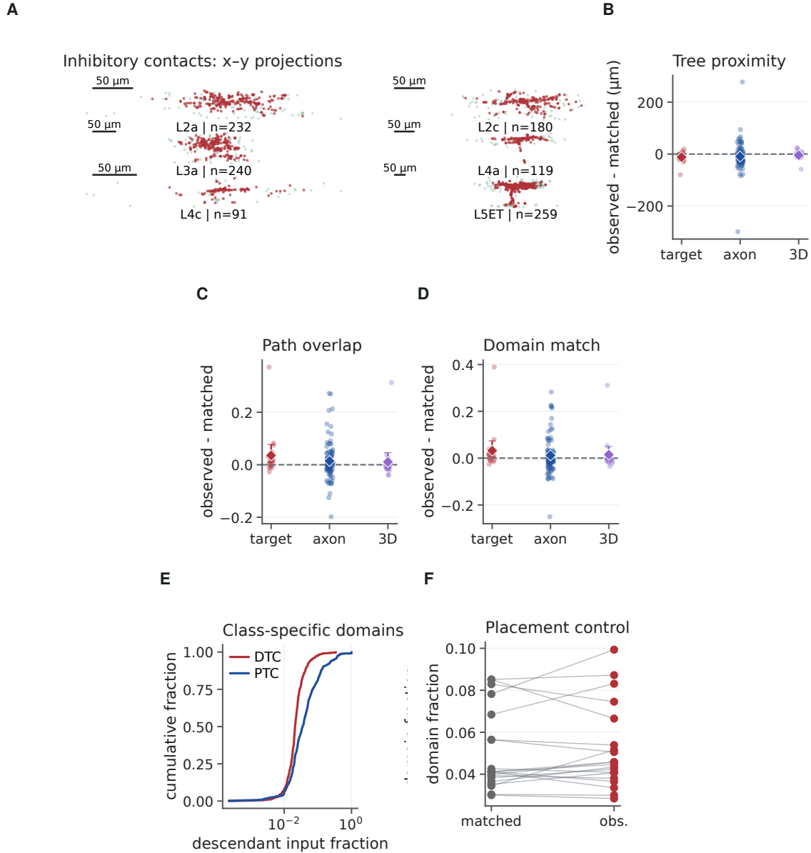
Figure S26: Spatial matching limits apparent inhibitory targeting of ancestry domains. A , Six layer-diverse reconstructions with mapped inhibitory contacts in x-y projection. B–D , Observed-minus-matched tree distance, shared-path fraction and weighted descendant-domain overlap in the twenty-target analysis, after aggregation within 92 presynaptic axons, and after joint path-distance/Euclidean matching. Symbols and intervals are means and 95% bootstrap intervals over the displayed inferential unit. Only tree distance persists after axon aggregation; no endpoint of the B–D triplet persists after joint three-dimensional matching. E , Cumulative descendant-input fraction by distal-dendrite-targeting versus perisomatic-targeting class, retaining one contact per axonal clump. F , Inhibitory-contact domain size versus matched locations; no reliable overall localization advantage is detected. Cells derive from one mouse. These structural comparisons do not show that contacts carried teaching signals.
