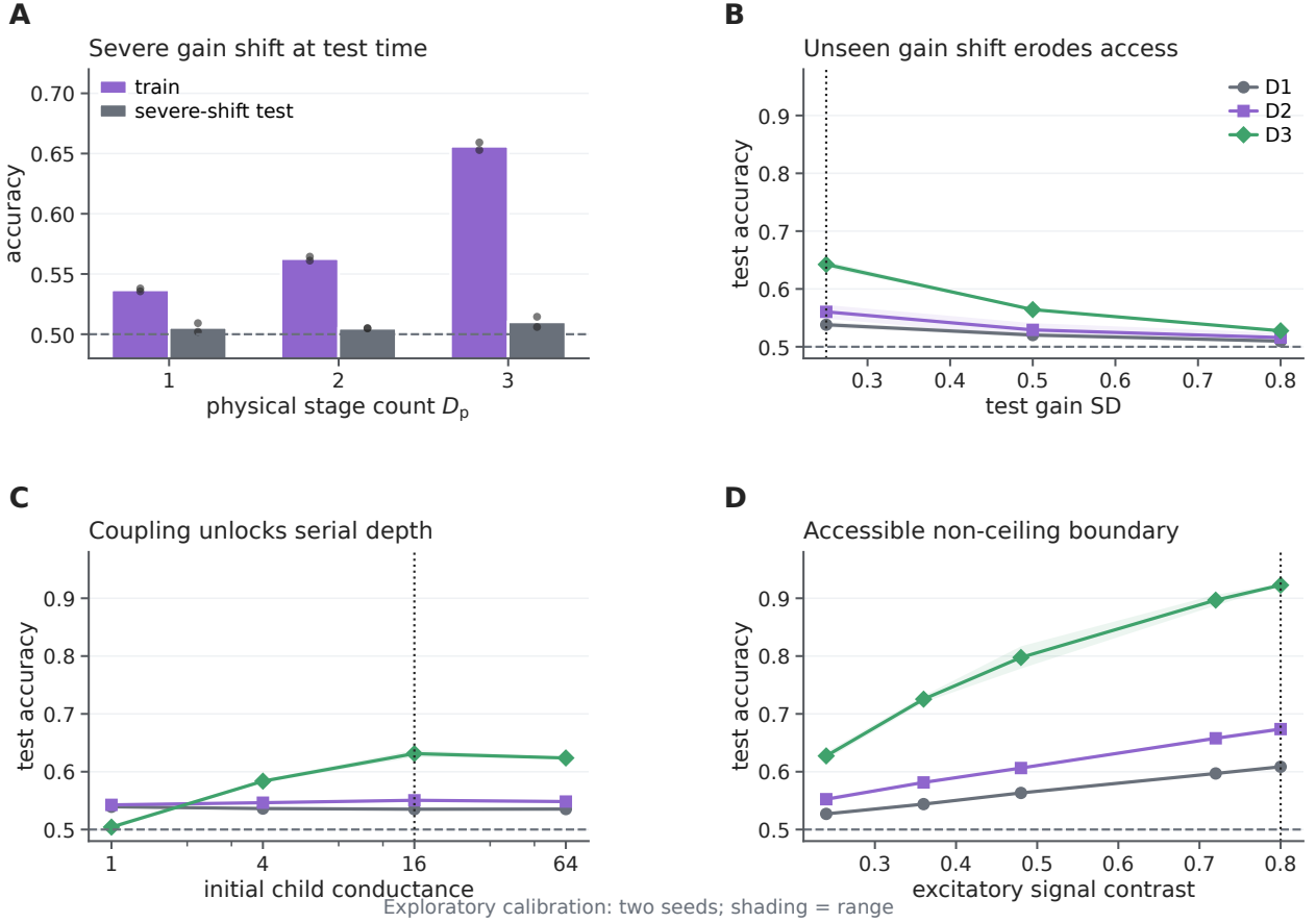
Figure S23: Transparent calibration of the nonlinear physical-depth operating point. All panels use the three-level hierarchical gain-load task and serial shunting morphologies D1 [8], D2 [2, 3] and D3 [2, 1, 2], each with eight nonsomatic compartments per soma. They test the prerequisite for the main hypothesis: whether the mechanism-matched divisive task is accessible at every depth before comparing depth benefits. A , The original aligned shunting-backpropagation (BP) pilot at signal contrast 0.24 fit the training distribution increasingly with depth but remained at chance under the prespecified severe gain shift (test gain standard deviation (SD) 1.2). Bars are two-seed means and dots are the individual exploratory seeds. B , With training gain SD fixed at 0.25, increasing unseen test gain variation eroded accessibility at every depth. The dotted line marks the matched train/test condition. C , At matched gain and signal contrast 0.24, stronger child coupling selectively made serial D3 computation accessible; the dotted line marks child conductance 16 used subsequently. D , At matched gain and child conductance 16, increasing excitatory signal contrast moved D1–D3 away from chance without saturating D1 or D2. The separately run 0.80 boundary (dotted line) met the predefined accessibility criterion and selected the operating point used for the analysis seeds. Lines show two-seed means; shading spans the two exploratory values and is not a confidence interval. All pilot, ladder and boundary seeds were excluded from the confirmatory contrasts.
