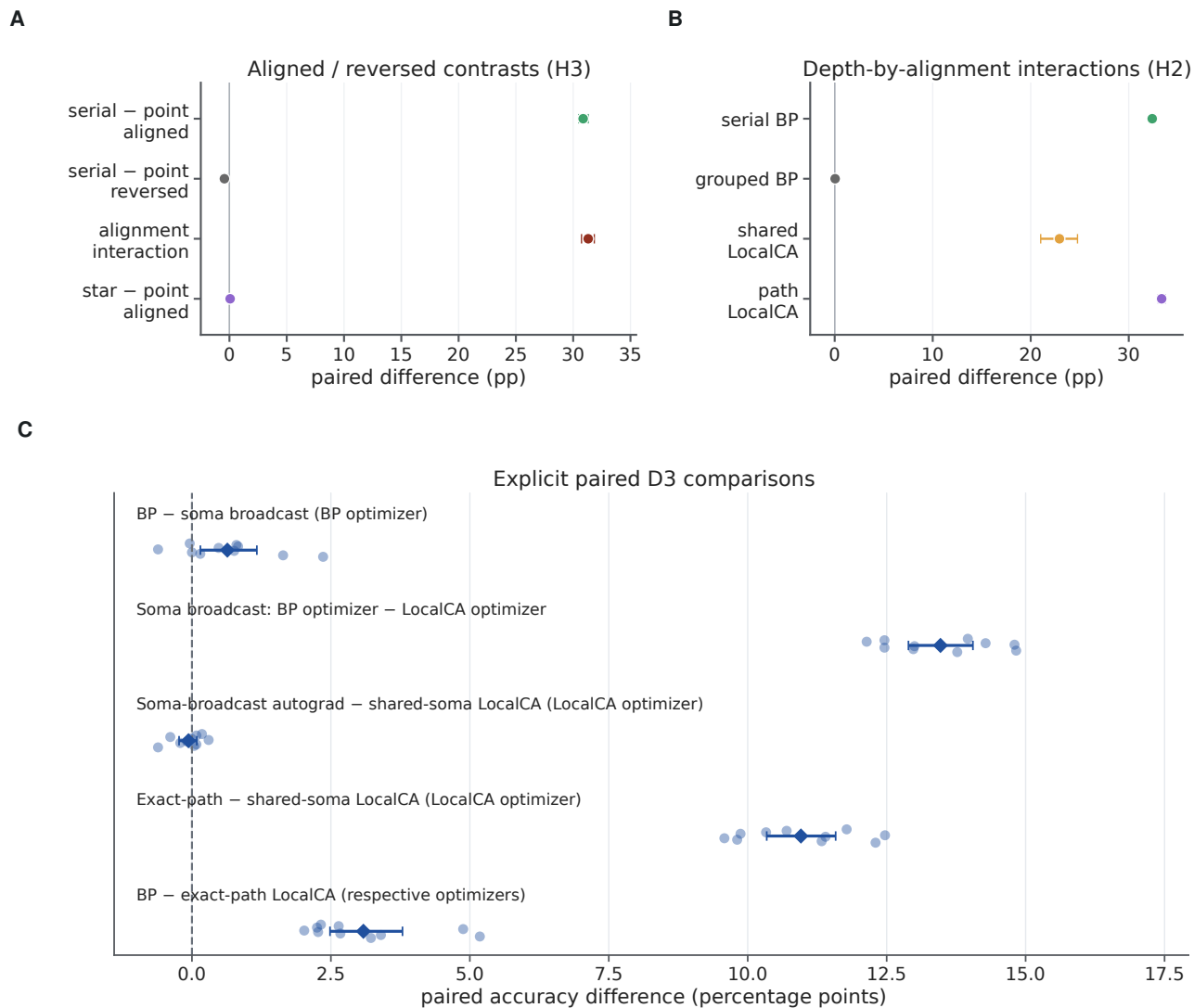
Figure S24: Physical-depth conclusions depend on alignment, task hierarchy and optimization. A , Serial/point contrasts under aligned and reversed placement. B , Separate independently seeded two-level task with D1 [8] and D2 [4, 1]: depth-by-alignment interactions for serial and grouped-point backpropagation and for shared or exact-path LocalCA. C , Original-budget D3 optimizer/credit-coordinate contrasts in the serial conductance morphology [2, 1, 2]. Under the BP optimizer, full versus soma-broadcast differentiation differs by 0.64 points; under the split LocalCA optimizer, exact versus shared differs by 10.96 points; changing the broadcast optimizer costs 13.47 points. Means and intervals use ten paired seeds and 95% bootstrap intervals. These earlier recipe-specific effects do not imply a converged credit advantage: at 600 epochs the LocalCA accuracy difference reverses, while exact credit retains lower cross-entropy (main Fig. 6). All D3 continuations hit the cap; D1 usually stops early.
