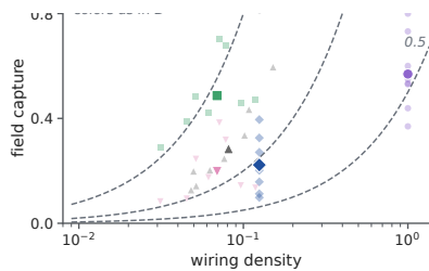
Wire efficiency at eight channels
