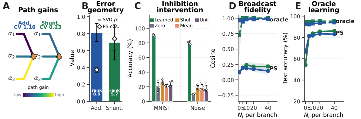
Figure 3: Mechanistic chain from path gains to learning. (A) Measured path-gain field. (B) MNIST exact-error geometry: rank-1 residual and actual per-soma broadcast cosine. (C) Post-training inhibitory-conductance interventions. (D,E) Broadcast fidelity and transported-error learning on noise resilience. Error bars are \pm 1 s.d.
