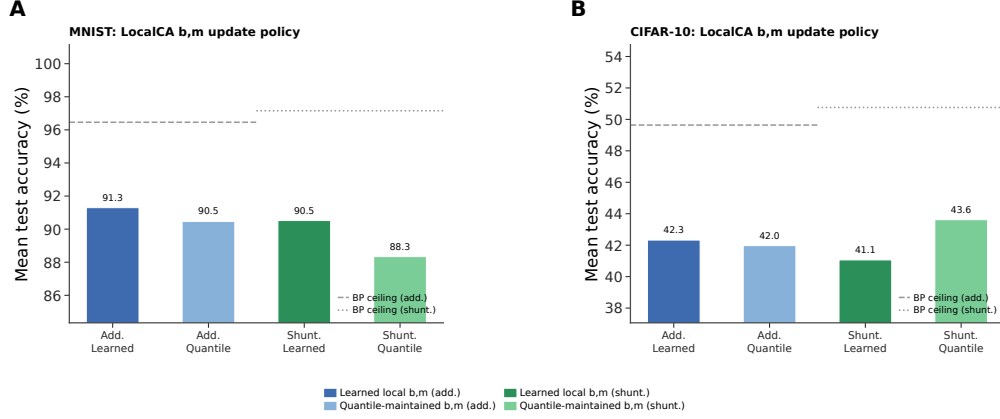
Figure S19: (b, m) update policy under quantile initialization. Each cluster of bars compares the mean test accuracy of learned local (b, m) and quantile-maintained (b, m) under LocalCA for additive and shunting cores, averaged across a matched morphology/init grid ( [2, 2] and [3, 3, 3] ; analytical and quantile init variants). Dashed and dotted horizontal lines mark the matched standard backpropagation ceiling for additive and shunting respectively. Left (MNIST): Learned local (b, m) is consistently better; quantile-maintained lags by 1.9 pp (additive) and 3.4 pp (shunting) on mean accuracy. Right (CIFAR-10): The gap reverses for shunting: quantile-maintained reaches 43.6% mean vs. 40.3% for learned local, while additive is essentially tied. The pattern suggests that quantile-maintained (b, m) prevents over-fitting the reactivation gate on harder inputs, making it a useful alternative in harder visual regimes.
