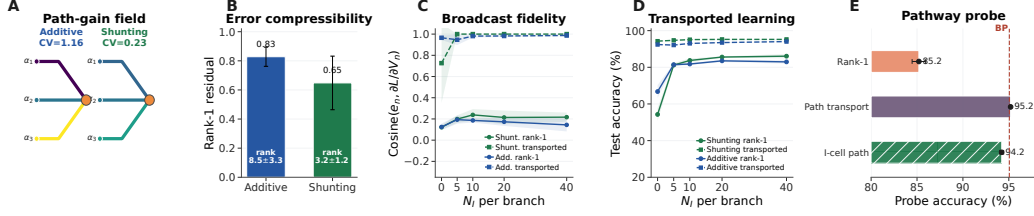
Figure 3: Mechanistic chain from path gains to learning. (A) Example dendritic path-gain field at matched inhibition, with measured MNIST CV annotated for additive and shunting networks. (B) Exact-error compressibility on MNIST: lower rank-1 residual and lower participation rank mean that a scalar broadcast is a better approximation. (C) Direct compartment-error fidelity on noise resilience. Solid lines compare rank-1 broadcast to the exact compartment error; dashed lines show the transported-error oracle. (D) Learning with the transported-error oracle. Improving the broadcast field recovers near-ceiling local learning, especially where rank-1 broadcast fails. (E) Compact inhibitory-path probe. In a one-layer noise-resilience test, exact path transport closes the rank-1 gap, and explicit inhibitory cells trained by the same local rule remain near the explicit-I backprop ceiling. Error bars denote \pm 1 s.d. across seeds.
