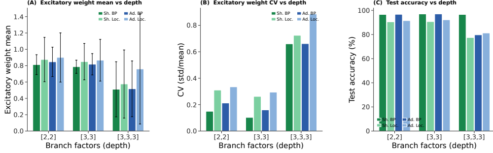
Figure S22: Synaptic weight statistics vs. dendritic depth (MNIST, 5 seeds/cell). (A) Excitatory weight mean (error bars = std). At [2, 2] and [3, 3], all four conditions cluster around 0.8–0.9; at [3, 3, 3] the means drop to \approx 0.5 –0.75 and the cross-seed spread grows, especially for additive LocalCA. (B) Coefficient of variation (CV = std/mean). At shallow/medium depth, LocalCA produces \sim 2\times higher CV than matched BP, but both remain well-behaved ( \leq 0.33 ). At the deepest network all four conditions jump to CV \approx 0.66 –0.88, with additive LocalCA the broadest. (C) MNIST test accuracy. BP tracks \sim 96 –97% at [2, 2]/[3, 3] and \sim 92 –95% at [3, 3, 3]. LocalCA stays within \sim 5 –6 pp of BP at shallow/medium depth but trails by \sim 15 –20 pp at [3, 3, 3], identifying depth as the remaining open challenge for this local rule. The qualitative ordering (shunting LocalCA tracks shunting BP more closely than additive LocalCA tracks additive BP) reinforces the manuscript claim that the conductance denominator is the key mechanistic ingredient.
