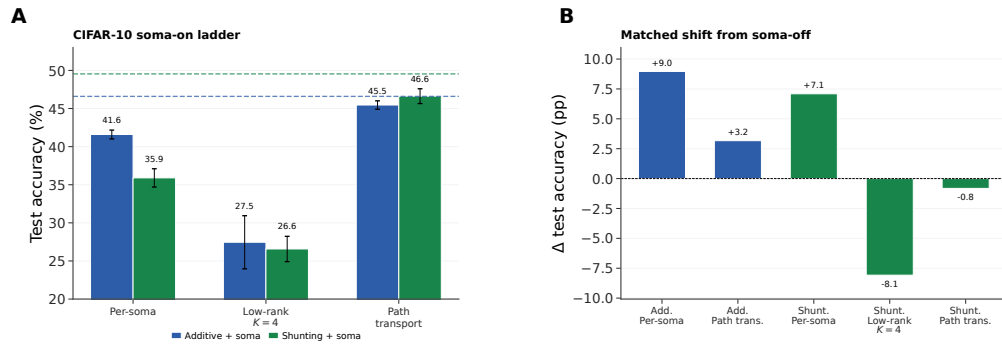
Figure S10: CIFAR-10 compact direct-I-stream depth-4 with somatic_synapses=true. (A) Absolute soma-on ladder on the compact direct-I-stream depth-4 family. Path transport stays strongest in both cores and remains near the matched backprop ceilings (dashed lines), while low-rank K=4 remains weak. (B) Matched shift from soma-off to soma-on for the conditions with a clean paired baseline. Soma helps additive strongly under per-soma and path transport, improves shunting per-soma, leaves shunting transported error close to its soma-off value, and worsens shunting low-rank K=4 . Additive low-rank K=4 is omitted from panel B because the soma-off mechanism package did not include that exact matched condition.
