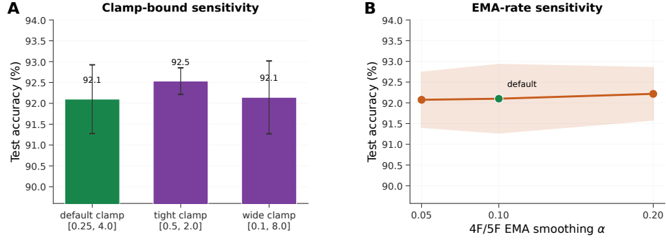
Figure S4: 5F sensitivity analysis (MNIST, shunting, per-soma broadcast) . (A) Sensitivity to the \phi_n clamp interval. The default clamp [0.25, 4.0] is already strong ( 92.1 \pm 0.8\% ); tightening it to [0.5, 2.0] slightly improves performance ( 92.5 \pm 0.3\% ), while widening it to [0.1, 8.0] is effectively neutral ( 92.1 \pm 0.9\% ). (B) Sensitivity to the 4F/5F EMA rate used for online statistics. Varying \alpha from 0.05 to 0.20 changes mean test accuracy by less than 0.2 pp. Together these results suggest that the 5F gain is not driven by a brittle single hyperparameter choice, even though the factor itself remains heuristic. Errors: \pm 1 s.d. across 3 seeds.
