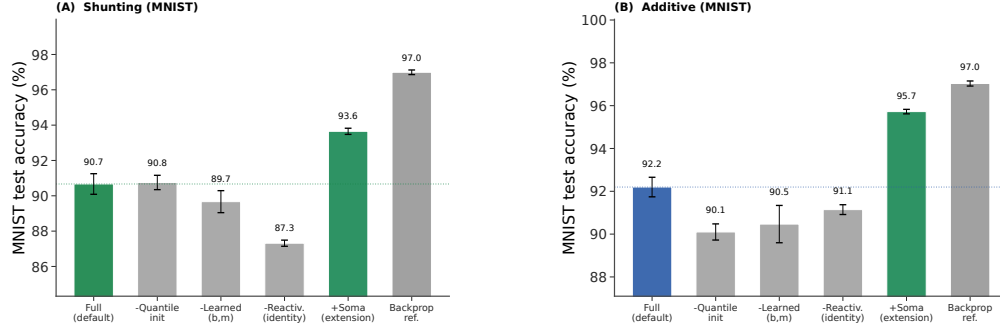
Figure S20: Per-component ablation for LocalCA on MNIST. Bars show mean test accuracy ( \pm s.d. across 5 seeds); coloured bars highlight the manuscript default (blue/green) and the soma-on extension (green). (A) Shunting: The full default reaches 90.7%; removing quantile init leaves accuracy unchanged at 90.8% (quantile init is a mild calibration nudge on this clean task), removing learned ( b, m ) drops by about 1 pp, and removing reactivation entirely drops accuracy to 87.3%; the reactivation transform is the largest single LocalCA ingredient. (B) Additive: Quantile init contributes +2.1 pp (90.1 \rightarrow 92.2%), learned ( b, m ) contributes +1.7 pp, and reactivation contributes +1.1 pp; each ingredient helps on the additive core. Soma-on is the largest positive change in both cores (+3 to +3.5 pp over full config), while matched standard backpropagation reaches 97.0% in both cores and sets the upper reference. The fixed-relu reactivation condition did not satisfy the same initialization checks and is omitted.
