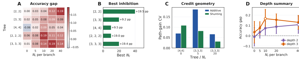
Figure S12: Morphology shifts the useful inhibitory regime. (A) Shunting-minus-additive LocalCA accuracy gap across dendritic morphologies and inhibitory synapse counts. (B) Best inhibitory count for each morphology. (C) Representative path-gain diagnostic for selected morphology cells, used to connect the performance map to credit geometry. (D) Average shunting advantage by depth, with markers showing the peak inhibitory count for each depth.
