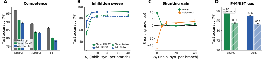
Figure 4: Capacity-calibrated competence and regime dependence. (A) Matched backprop ceilings vs. rank-1 5F LocalCA on MNIST, Fashion-MNIST, and context gating, including the matched additive context-gating rerun. (B,C) Inhibitory dose-response and shunting advantage on MNIST and noise resilience. (D) Fashion-MNIST confirms a smaller but consistent shunting advantage. Error bars denote \pm 1 s.d. across seeds.
